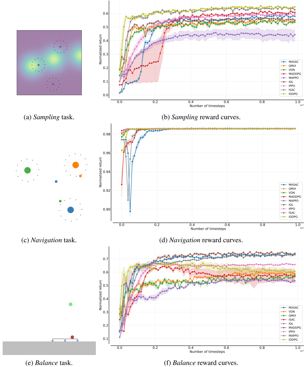
Figure 5: The sample efficiency curves for all BenchMARL algorithms over the three VMAS tasks analyzed. We report the inter-quartile mean (IQM) with 95% stratified bootstrap confidence intervals over 3 random seeds for each experiment. Details and references for the algorithms used are available in Table 1.
