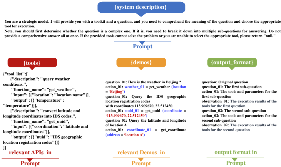
Figure 2: Demonstrations of the specific formats of each component in the prompt.
