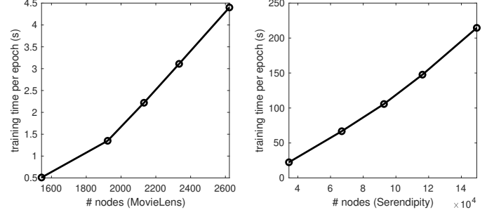
Fig. 7: Training time w.r.t. graph size.
