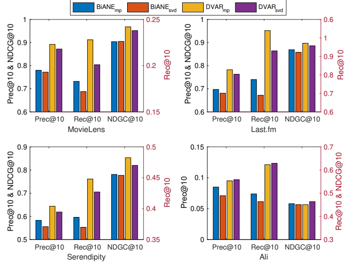
Fig. 5: Impact of feature initialization.
