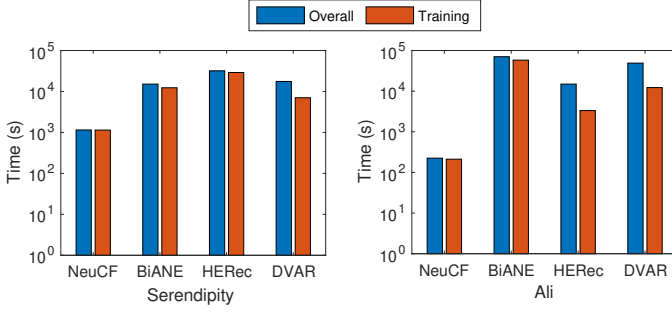
Fig. 8: Efficiency study on Serendipity and Ali dataset.
