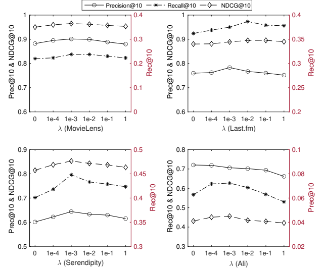
Fig. 4: Impact of \lambda .
