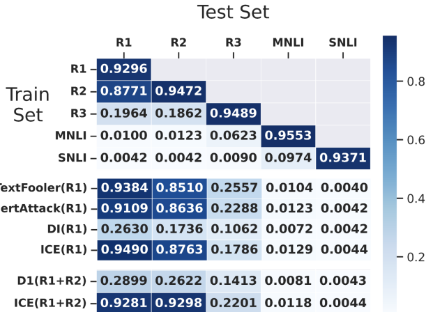
Figure 2: Distributional similarity, as measured by MAUVE on RoBERTa embeddings from a random 1k sample (Pillutla et al., 2021). MAUVE scores range from 0 to 1, with higher values indicating more similar distributions. MAUVE metrics are intended to be evaluated relative to each other, and not as absolute measures. Note that distributional similarity to the held out attacks, R2, does not correlate with whether an attack generation method is useful as per Table 1.
