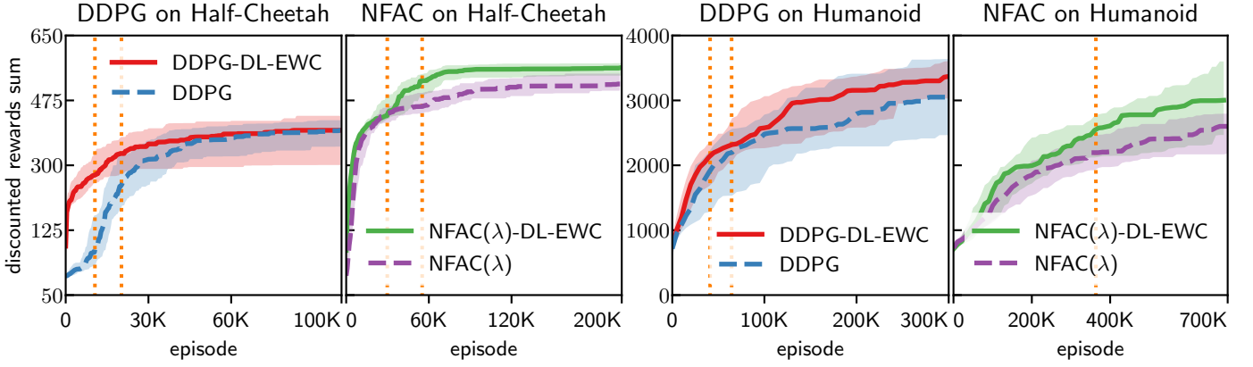
Fig. 5. Median and quartiles of the best registered performance during the testing phase with NFAC( \lambda ) and DDPG on Half-Cheetah and Humanoid environments. When the DL are added, EWC is used to help the transfer. The averages of the transfer moments are displayed vertically (dashed orange).
