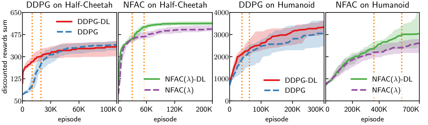
Fig. 6. Median and quartiles of the best registered performance during the testing phase with NFAC( \lambda ) and DDPG on Half-Cheetah and Humanoid environments. When the DL are added, only the “initialization” method is used to transfer. The averages of the transfer moments are displayed vertically (dashed orange).
