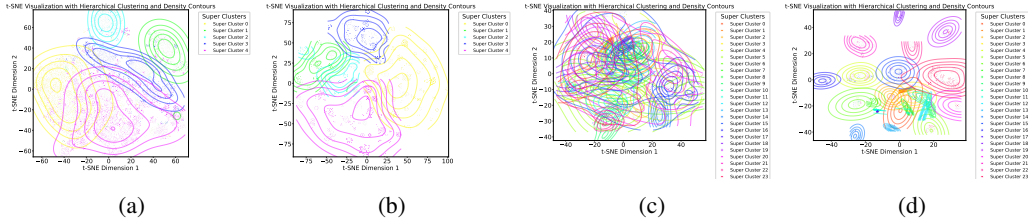
Figure 2: Embedding visualizations for different datasets, projected using t-SNE for dimensionality reduction. The density contours represent the kernel density estimation (KDE) of the embeddings in the 2D space, highlighting the clustering structure. Subplots show the Material dataset (a) before and (b) after model alignment, and the Healthcare dataset (c) before and (d) after model alignment. The contours illustrate the density distribution of embeddings, showcasing the effect of alignment on cluster compactness and separation.
