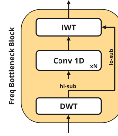
Figure 4: Overview of Frequency Bottleneck Block
