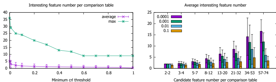
Fig. 2. Number of interesting features per comparison table
