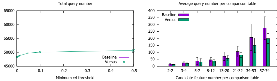
Fig. 3. Number of SPARQL queries executed on Wikidata
