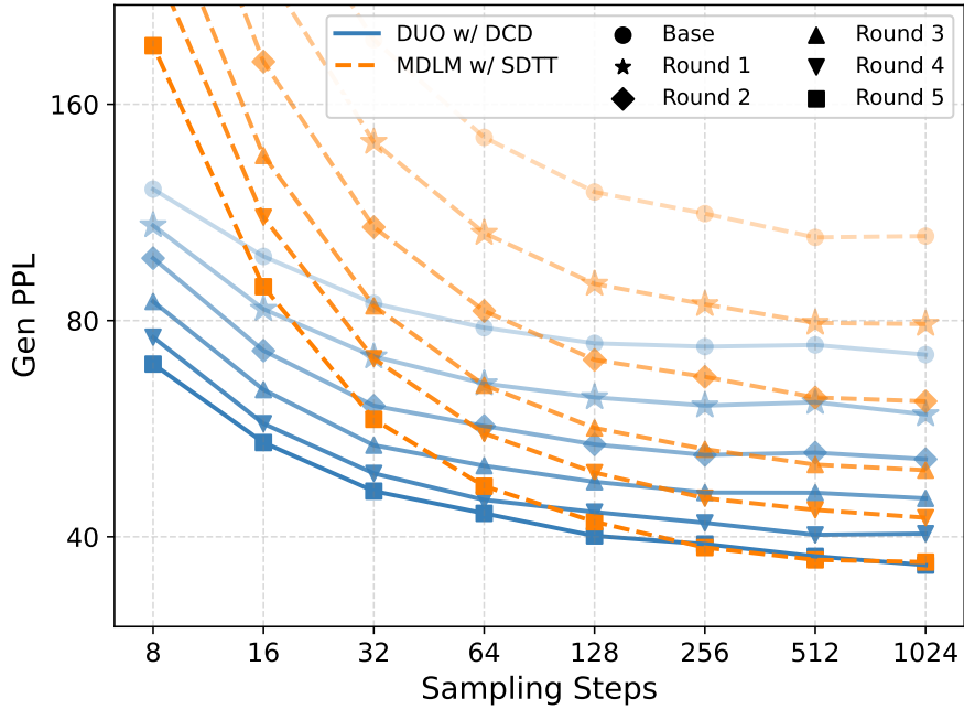
Figure 12: Sample quality comparison using Gen PPL ( \downarrow ) of Duo (Ours) distilled with our proposed DCD algorithm and MDLM distilled with SDTT after successive distillation round. Duo always dominates in the low sampling steps regime. Refer Table 7 for the exact quantitative numbers.
