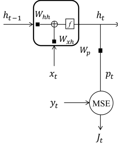
Figure 4.2: Forward propagation of a RNN at a time step t . The state \mathbf{h}_t , the forecast \mathbf{p}_t and the error \mathbf{J}_t are updated with parameters unchanged, such as weights \{\mathbf{W}_{hh}, \mathbf{W}_{xh}, \mathbf{W}_p\} and bias \{\mathbf{b}_{hh}, \mathbf{b}_{xh}, \mathbf{b}_p\} , during forward propagation..
