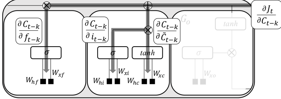
Figure 4.13: Back-propagating error through state C_{t-k} . Forget and input gate, G_f and G_i involve in this backpropagation. Gradients in terms of parameters can be expressed by the chain rule that is derived from the partial derivative of an error j_t with respect to C_{t-k} and others depending on the parameters.
