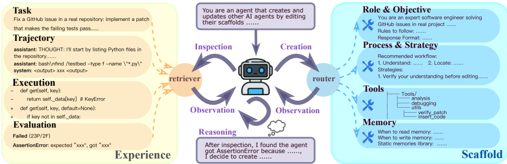
Figure 3: The pipeline of ReCreate framework. ReCreate-Agent iteratively reasons and acts to locate key evidence on why the agent succeeds or fails and reflect how to improve the agent scaffold.
