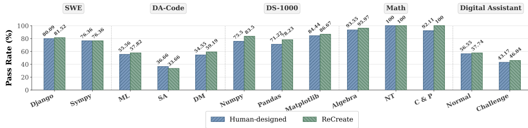
Figure 9: ReCreate on various base models for ReCreate Agent.
