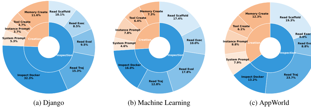
Figure 6: Action distributions of the ReCreate-Agent in various domains.
