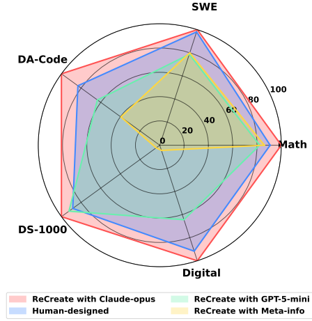
Figure 5: Reasoning-level Ablation.
