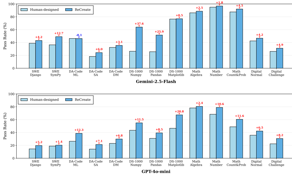
Figure 10: ReCreate on various base models for task agent.
