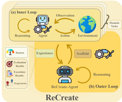
Figure 2: The overview of ReCreate.
