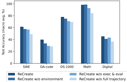
Figure 4: Ablations on experience components.
