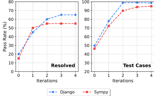
Figure 7: Post-update Gain on SWE tasks.
