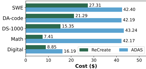
Figure 8: Cost Comparison (USD).
