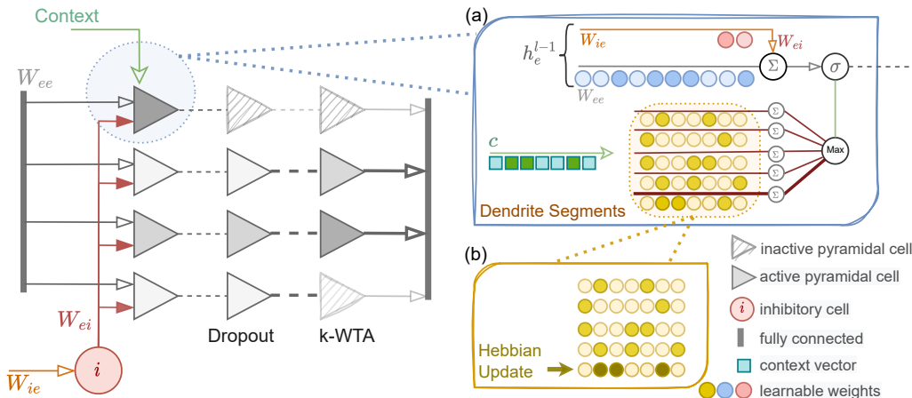
Figure 1: Architecture of one hidden layer in the biologically plausible framework. Each layer consists of separate populations of exclusively excitatory pyramidal cells and inhibitory neurons which adheres to Dale’s principle. The shade indicates the strength of weights or activations where darker shade indicating higher value. (a) The pyramidal cells are augmented with dendritic segments which receive an additional context signal c and the dendrite segment whose weights are most aligned with the context vector (bottom row) is selected to modulate the output activity of the feedforward neurons for context-dependent processing of information. (b) The Hebbian update step further strengthens the association between the context and the winning dendritic segment with maximum absolute value (indicated with darker shade for bottom row). Finally, Heterogeneous dropout keeps the activation count of each pyramidal cell (indicated with the gray shade) and drops the neurons which were most active for the previous task (darkest shade dropped) to enforce non-overlapping representations. The top-k remaining cells then project to the next layer (increased shade).
