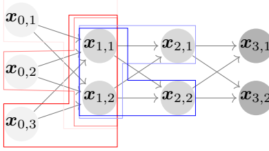
Figure 1: A toy BNN with L = 2 and (n_0, n_1, n_2, n_3) = (3, 2, 2, 2) . The subsets of interacting variables I_1 = \{x_{0,1}, x_{1,1}, x_{1,2}\} , I_2 = \{x_{0,2}, x_{1,1}, x_{1,2}\} , I_3 = \{x_{0,3}, x_{1,1}, x_{1,2}\} (represented by red polygons) and I_4 = \{x_{1,1}, x_{1,2}, x_{2,1}\} , I_5 = \{x_{1,1}, x_{1,2}, x_{2,2}\} (represented by blue polygons) are used to compute \tau_{\text{tighter,cs}}^1 .
