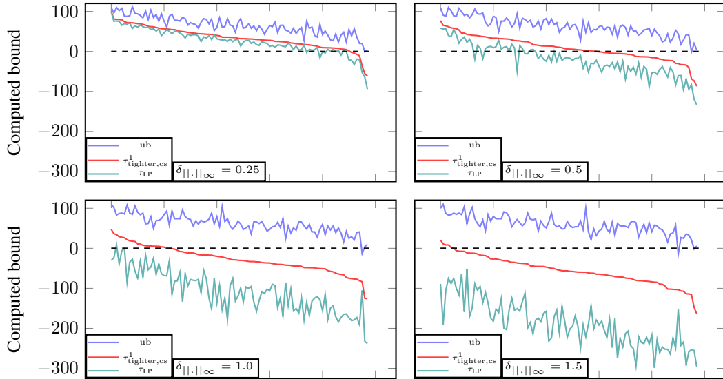
Figure 2: Comparing \tau_{\text{LP}} and \tau_{\text{tighter,cs}}^1 bounds for \text{BNN}_1 and different \delta_{\|\cdot\|_\infty} . Each subplot x -axis represents indices of test set images sorted in the descending order of \tau_{\text{tighter,cs}}^1 values. The upper bound \text{ub} is obtained by random sampling. The relative improvement over LP is estimated through \frac{\tau_{\text{tighter,cs}}^1 - \tau_{\text{LP}}}{\text{ub} - \tau_{\text{LP}}} . On average, \tau_{\text{tighter,cs}}^1 bounds are 21, 33, 46 and 53 percent more accurate, respectively.
