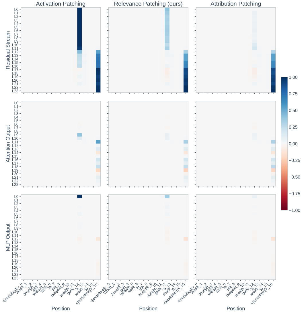
Figure 5: Qualitative comparison showing how accurately relevance patching (ReP) and attribution patching (AtP) approximate the effects of activation patching in Pythia-410M. ReP shows notably better alignment in the residual stream and at MLP0, where AtP’s estimates are less reliable.
