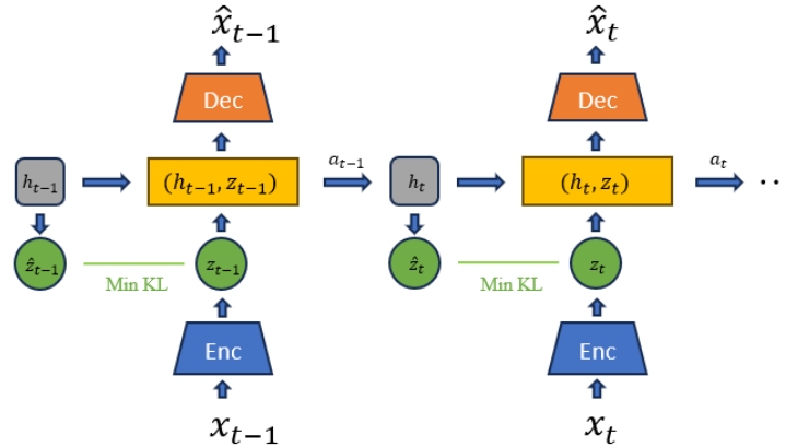
Figure 8: RSSM Structure
