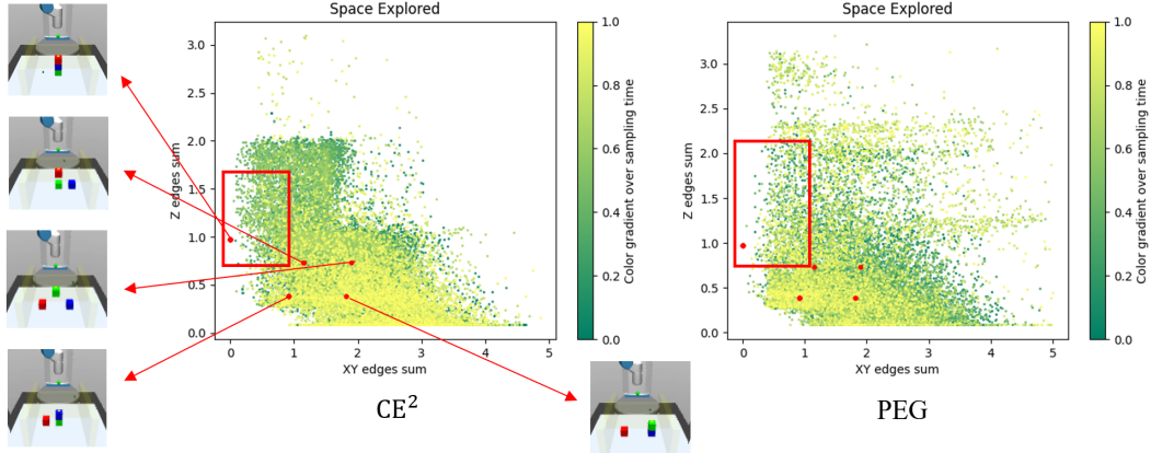
Figure 10: Space explored by CE^2 and PEG in the 3-Block Stacking environment at 1M steps. X-axis: the sum of the three sides of the triangle projected on the x-y plane by the three block-connected triangles. Y-axis: sum of heights (z-coordinates) of the three blocks. Red points: evaluation goals. Other points: observations of trajectories sampled in real environment. Color from green to yellow means to be sampled more recent.
