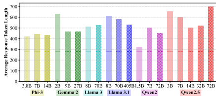
Figure 7: Average Output Length of synthetic datasets generated using different response generators (measured in Tokens).
