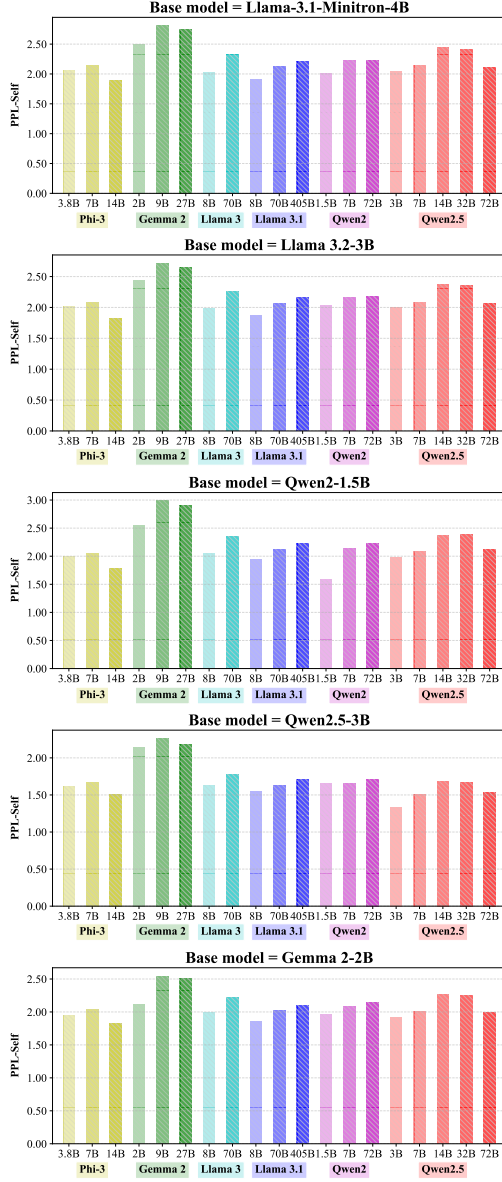
Figure 9: PPL-Self of five base models.
