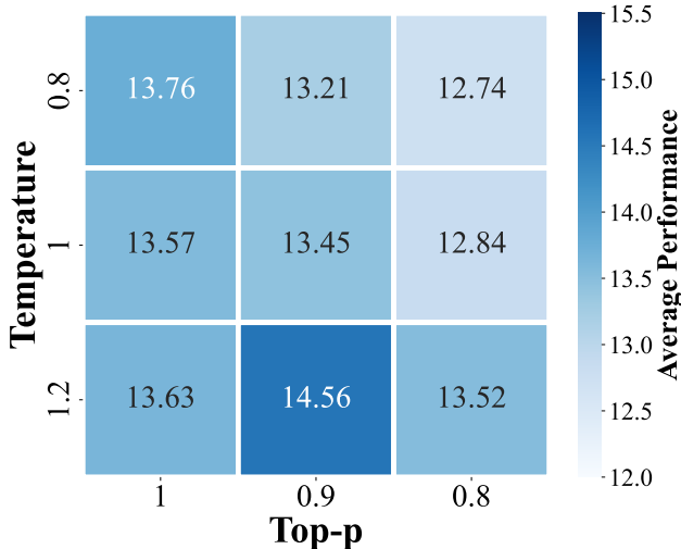
Figure 5: This figure demonstrates the impact of different sampling hyper-parameters when generating responses. We use Gemma-2-9b-it as the response generator. All models are supervised-fine-tuned on the Llama-3.1-Minitron-4B base model.
