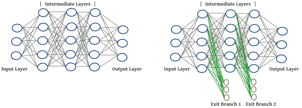
Fig. 2. Illustration of conventional DNN (left) and early-exit DNN (right) with two side branches.
