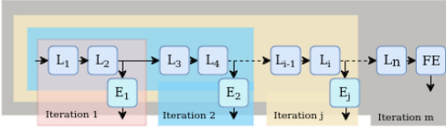
Fig. 6. A visual representation of the separate training strategy.
