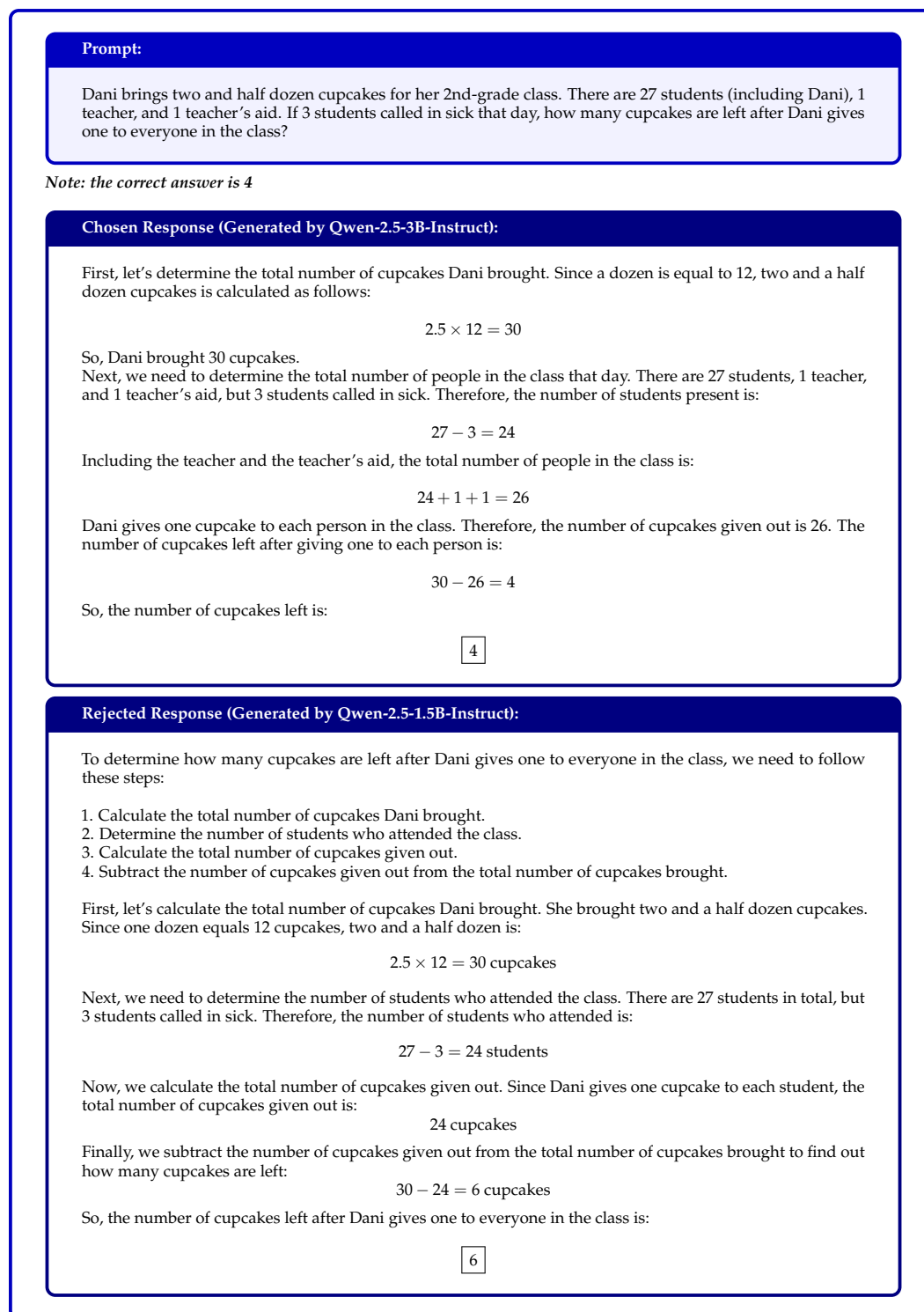
Figure A3: Qualitative example of a preference pair from our Qwen 3B over 1.5B weak preference data. On this math prompt (ground-truth answer is 4 cupcakes), the Qwen 3B-generated chosen response contains a verifiably correct answer, while the Qwen 1.5B-generated rejected response is incorrect (6 cupcakes).
