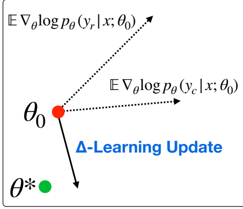
Figure 4: We train student model \theta_0 to prefer pseudo-labels y_c from a (possibly weak) teacher model \theta_c over pseudo-labels y_r from a weaker teacher \theta_r . Individually, the gradient updates \nabla_{\theta} \log p_{\theta}(y_c | x; \theta_0) , \nabla_{\theta} \log p_{\theta}(y_r | x; \theta_0) (dashed arrows) induced by the weak labels can be harmful in expectation and steer the student away from the ground-truth parameters \theta^* . In contrast, the delta learning gradient updates follow their difference vector \nabla_{\theta} \log p_{\theta}(y_c | x; \theta_0) - \nabla_{\theta} \log p_{\theta}(y_r | x; \theta_0) , which is positively aligned with \theta^* whenever \theta_c outperforms \theta_r . Pairing weak-and-weaker teachers thus yields a learning signal that can improve a stronger student.
