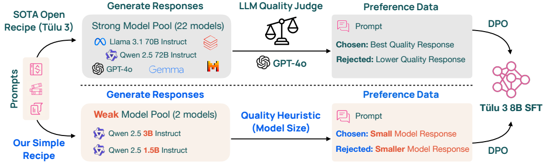
Figure 2: We simplify the Tülu 3 preference data recipe (top half). Instead of using a GPT-4o judge to pick the best response from many strong models as chosen, our recipe (bottom half) uses a single small model to generate all chosen responses, relying on the implicit delta to an even smaller (and thus weaker) model’s responses to drive downstream learning.
