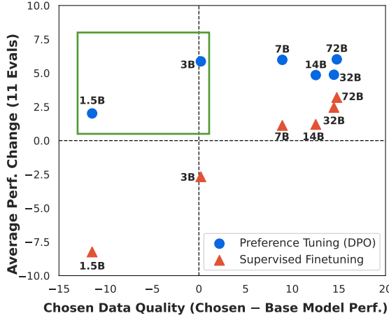
Figure A2: Impact of chosen data quality : We plot the performance of the model used to generate chosen responses ( x -axis) against performance change after tuning on those responses ( y -axis). SFT only yields gains when training on responses from models stronger than the base model we tune from; gains scale with chosen quality. DPO yields gains even when the chosen responses come from models no stronger than the base ( green box ); increasing chosen response quality gives quickly diminishing returns. Each dot represents a model tuned on chosen responses generated by a Qwen 2.5 Inst. model (parameter size labeled).
