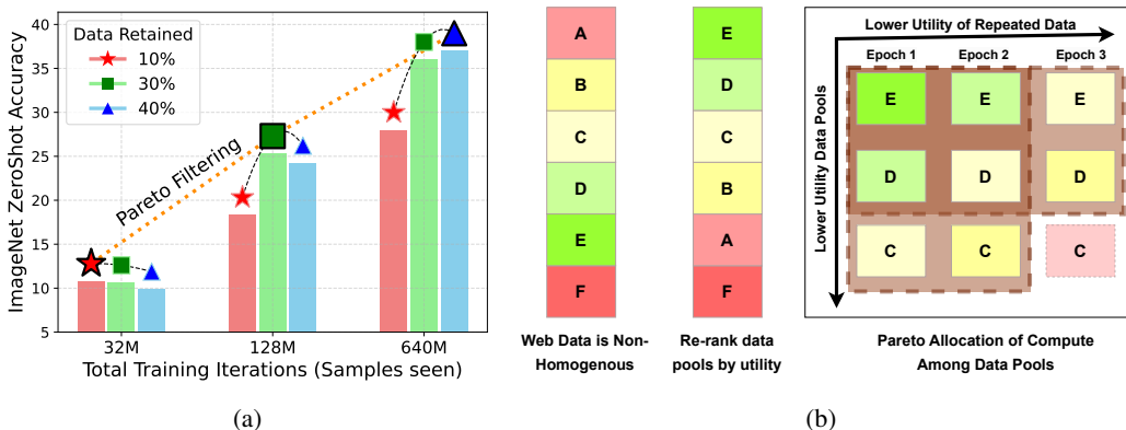
Figure 1: (a) Retaining top-30% data based on CLIP score is common in vision-language model training. Our results show that filtering thresholds must adapt to the compute-to-data pool ratio, accounting for the diminishing utility of good data with repetitions. Results on pretraining on a 128M sample global data pool at different compute scales. (b) The Dynamic Problem of Data Filtering: Web data is non-homogenous, and past work has succeeded at ranking various data subsets according to their diminishing quality (y-axis). However, training on ‘high-quality’ data for multiple epochs leads to diminishing utility (x-axis), an angle ignored in past work. In this dynamic environment, what is the best allocation of and return for computational resources?
