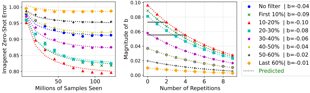
Figure 3: Scaling curves with repeated data for visual-language models: We partition DataComp medium scale pool samples into buckets, based on their CLIP scores, and train a model on each bucket for 10 epochs. (a) Estimated error curves using the proposed scaling laws (Equation 5). (b) Diminishing utility with epochs of various data subsets. Observe that the utility of the best bucket (red) at it’s 4 th repetition becomes less than that of worse buckets like top-30%-40% subset.
