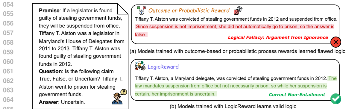
Figure 1: Comparison between models trained on data constructed with outcome-based or probabilistic process rewards and those trained with LogicReward.
