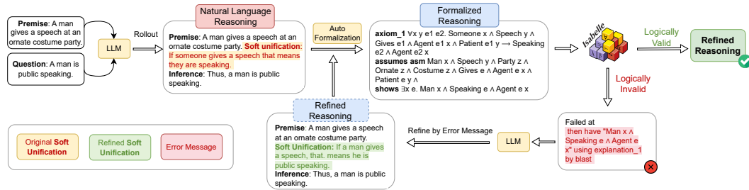
Figure 3: We present an illustrative example of leveraging Isabelle’s error messages to refine the Soft Unification process. For simplicity, we show a single-step example.
