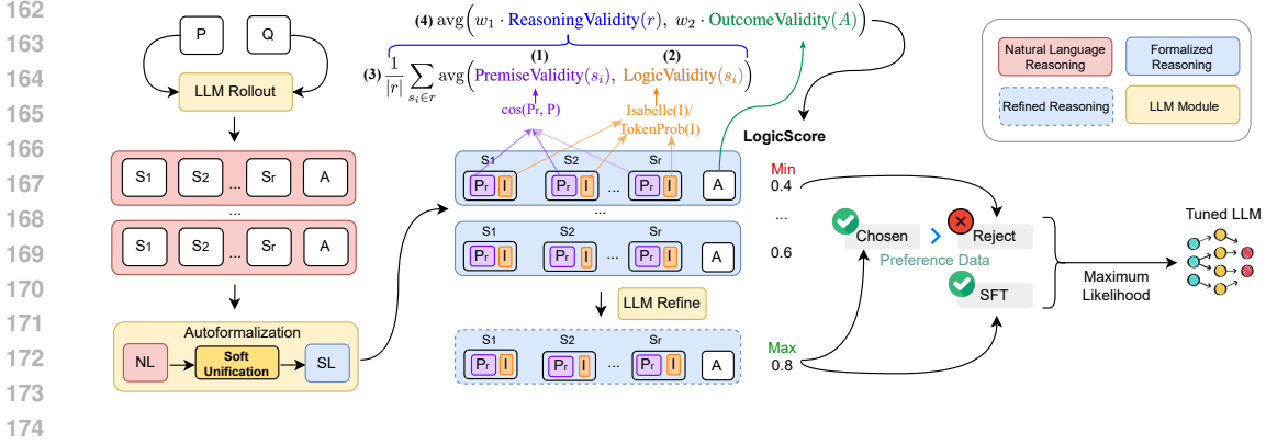
Figure 2: LogicReward Pipeline. We begin by rolling out responses with LLMs, followed by Autoformalization with Soft Unification. Each response is first assigned a Premise Validity score by comparing the used premises P_r with the given premises P , after which Logic Validity checks inference I using Isabelle. These are combined into Reasoning Validity, which is further integrated with Outcome Validity to yield the final LogicScore. The highest-LogicScore response is used to construct SFT data, while the responses with maximum and minimum LogicScores are paired to create DPO data for training.
