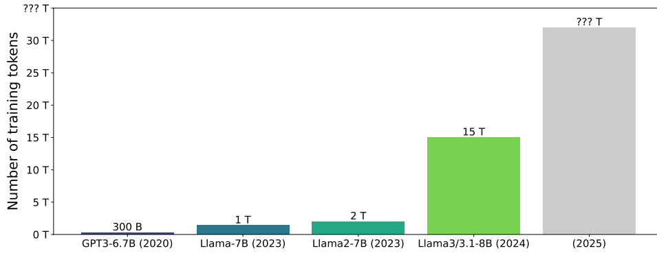
Figure 13: The number of training tokens for the state-of-the-art 7B-scale LLMs increase by nearly 50× over the past 4 years. According to this trend, it is expected that the future 7B models will have much more training tokens.
