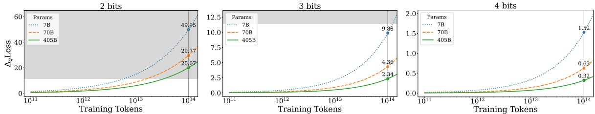
Figure 12: Scaling laws for predicting Quantization-induced Degradation (QiD) , denoted as \Delta_q Loss in 7B, 70B, and 405B models trained on up to 100 trillion ( 10^{14} ) tokens. While low-bit quantization yields acceptable QiD for undertrained LLMs (trained with \leq 10^{12} tokens), it is predicted to become undesirable when applied to fully trained LLMs (e.g., trained with 100 trillion tokens, a milestone expected to be reached in the next few years), particularly for smaller models. Note that the gray areas in this figure indicate levels of QiD that degrade the model’s predictions to a level worse than random guessing.
