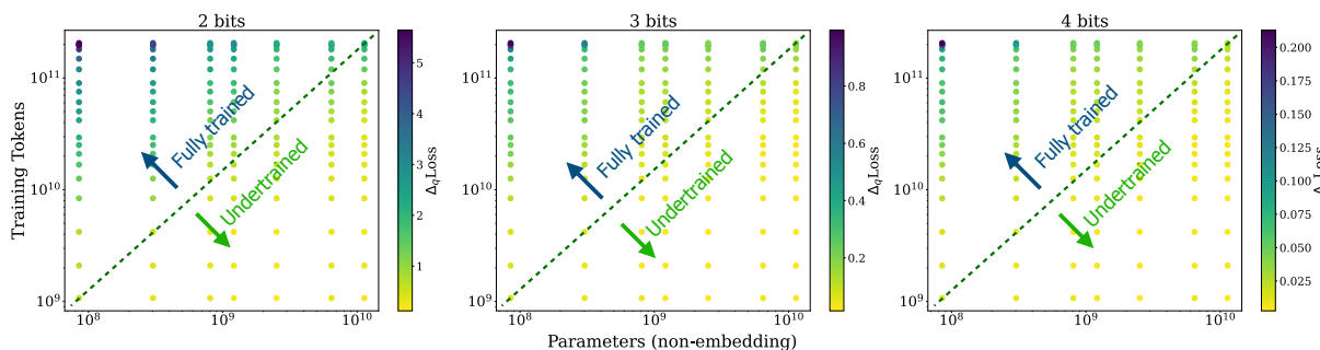
Figure 10: Fully trained LLMs suffer from much greater QiD (i.e., \Delta_qLoss ) than undertrained LLMs.
