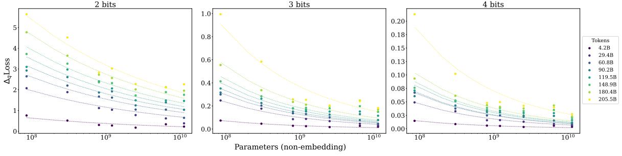
Figure 3: The fitted scaling law of QiD with respect to the model size (i.e., the number of non-embedding parameters) in the form of Equation 6, where \alpha is fitted to be 0.2276.
