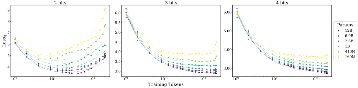
Figure 6: We can predict the performance of a quantized LLM as Loss_q = Loss_{16-bit} + \Delta_q Loss , where Loss_{16-bit} can be predicted by the conventional LLM’s scaling law which is fitted based on the function form of Equation 3 with the LLMs in the Pythia suite as Loss_{16-bit} = [(4.74e^{19}/N)^{(0.045/0.399)} + 7.63e^{10}/D]^{0.399} .
