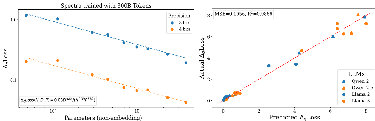
Figure 9: Left: Scaling laws for low-bit quantization, fitted on the LLM checkpoints of the Spectra suite, which are all trained with 300B tokens; Right: Actual \Delta_qLoss VS Predicted \Delta_qLoss that is computed based on the scaling laws fitted on Llama and Qwen.
