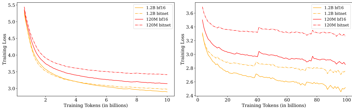
Figure 14: Training losses of BitNet and its 16-bit counterparts show a trend similar to that of low-bit quantization – they tend to perform well when undertrained but struggle to match the performance of fully trained LLMs.
