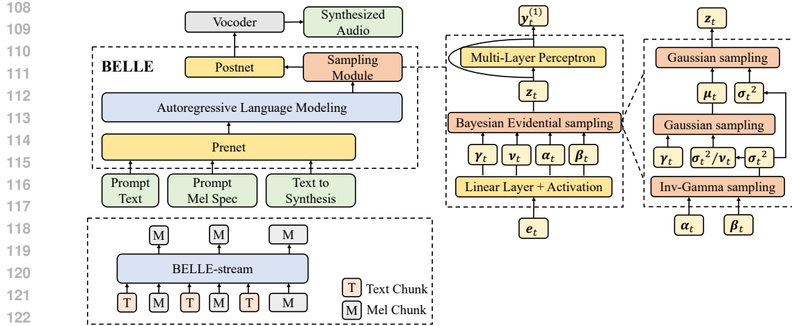
Figure 1: The structure of BELLE and the detailed sampling module. The output is assumed following a Normal-Inverse-Gamma (NIG) distribution and Sampling Module predicts four distribution parameters. Sequentially, variance and mean are obtained via Inverse-Gamma sampling and Gaussian sampling, respectively, followed by a final Gaussian sampling step to generate the output \mathbf{y}_t^{(1)} . BELLE-stream adopts the same architecture as BELLE. The text and Mel-spectrogram are split into chunks and interleaved to form the input sequence. Typically, the final chunk generates all remaining audio, making it longer than the preceding ones.
