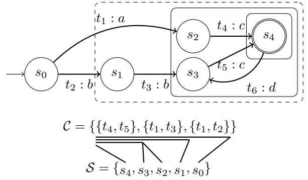
Figure 3: Transition system with cost(t_1) = 2 and cost(t_i) = 1 for i > 1 . Boxes around states show the goal zone after each iteration. Transitions entering a goal zone are part of the cut. In the disjoint variant, the dashed cut is not found. Below is the set \mathcal{C} of discovered cuts and our data structure mapping states s \in \mathcal{S} to sets of s -cuts.
