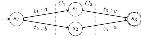
Figure 2: Example transition system with two cuts C_1 and C_2 . Transition labels give transition and operator, separated by a colon.
