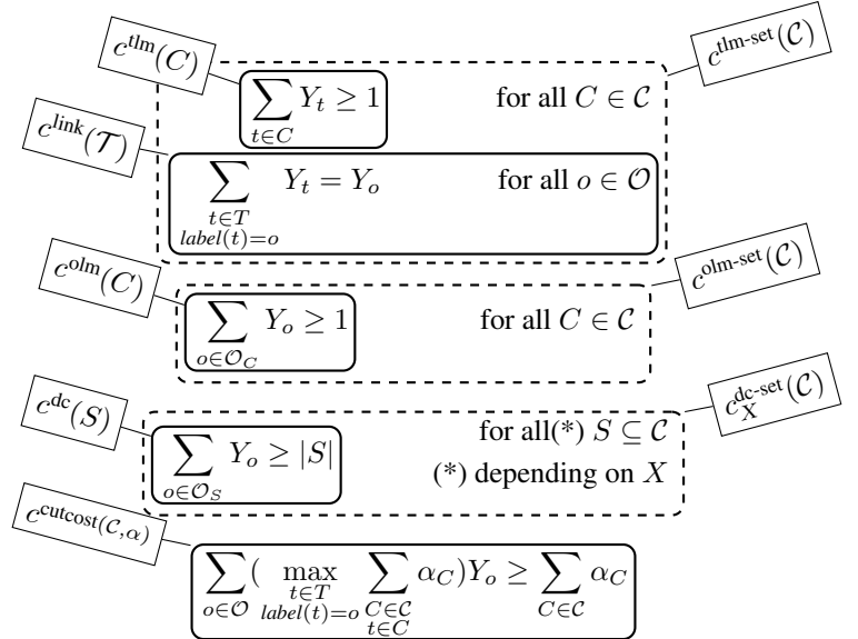
Figure 1: Cut-based constraints introduced in the paper.
