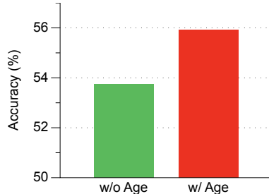
Figure 3: Imputing features with real data, i.e., Age. We report the mean accuracy (%) across three random splits on the Clinical dataset using XGBoost.
