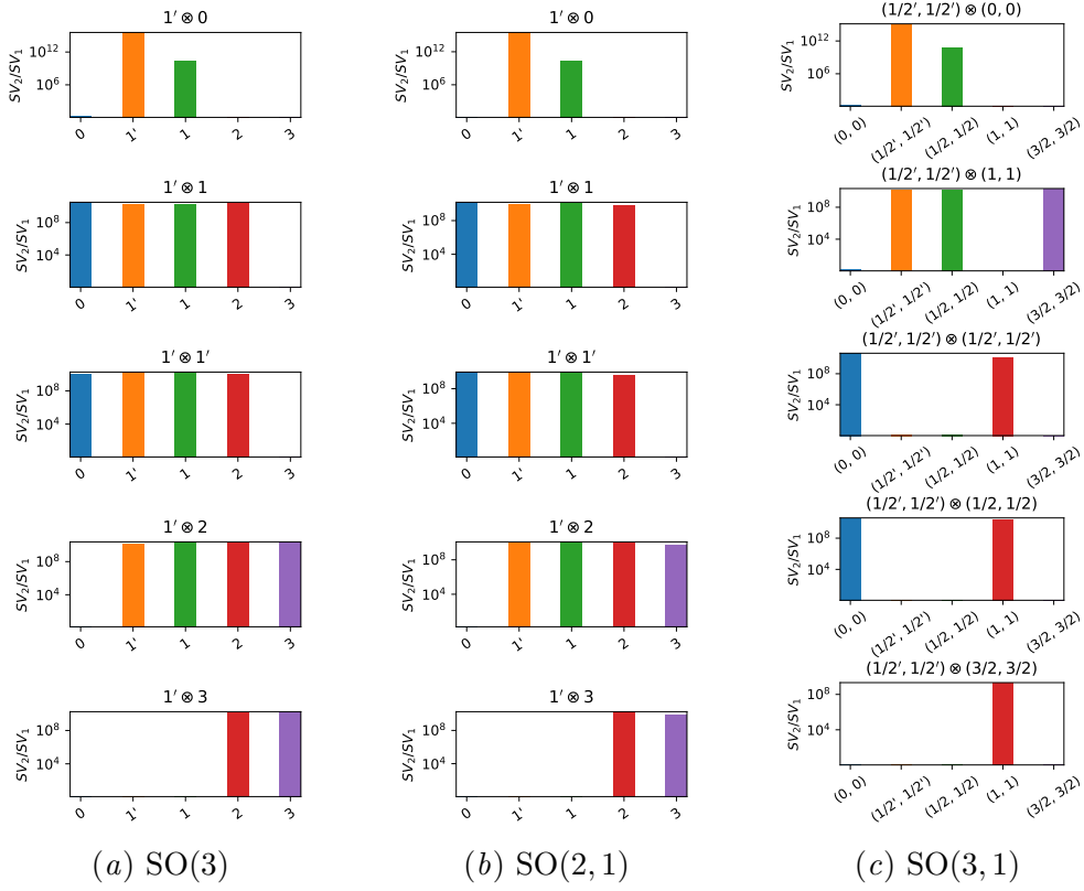
Figure 3: Tensor product structure of the learned group representations \rho with several known (analytically-derived) group representations \rho_1 for the groups \text{SO}(3), \text{SO}(2,1) , and \text{SO}(3,1) . Each column is for the group indicated at the bottom, each row is for a different choice of \rho_1 for that group, and the horizontal axis indicates the \rho^{(i)} onto which we project the tensor product \rho \otimes \rho_1 \cong \bigoplus_{i \in I} \rho^{(i)} . The diagnostic r (defined by eq. (7) in section 2.5) is plotted on the y -axis with a log scale for each subfigure. The labelling of group representations is explained in section 4, recall that the primed integers indicate learned representations. The first row demonstrates by Schur's Lemma that to within numerical error of about \sim 10^{-6} the learned \text{SO}(3) group representation denoted 1' is isomorphic to the spin-1 irreducible group representation obtained from known formulae, i.e. 1'_{\text{SO}(3)} \cong 1_{\text{SO}(3)} . The first row also indicates that 1'_{\text{SO}(2,1)} \cong 1_{\text{SO}(2,1)} , and (1/2', 1/2')_{\text{SO}(3,1)} \cong (1/2, 1/2)_{\text{SO}(3,1)} . The remaining rows indicate that the tensor product structure of the learned group representations matches that of the known irreducible group representations.
