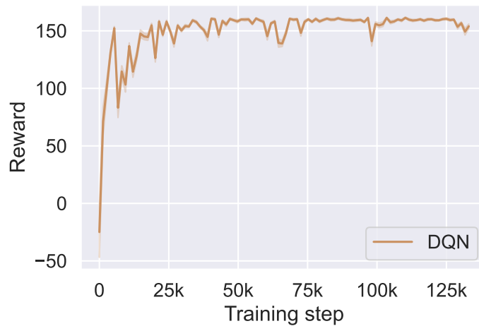
Figure 18: Learning curves of DQN on WDSEnv.
