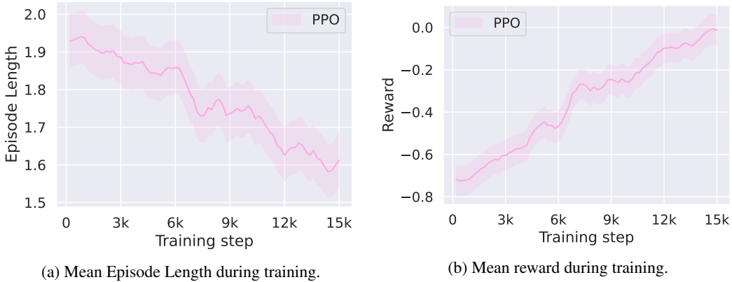
Figure 12: RoboFeeder-picking-v0, PPO training curve of mean episode length and reward over 5 seeds.
