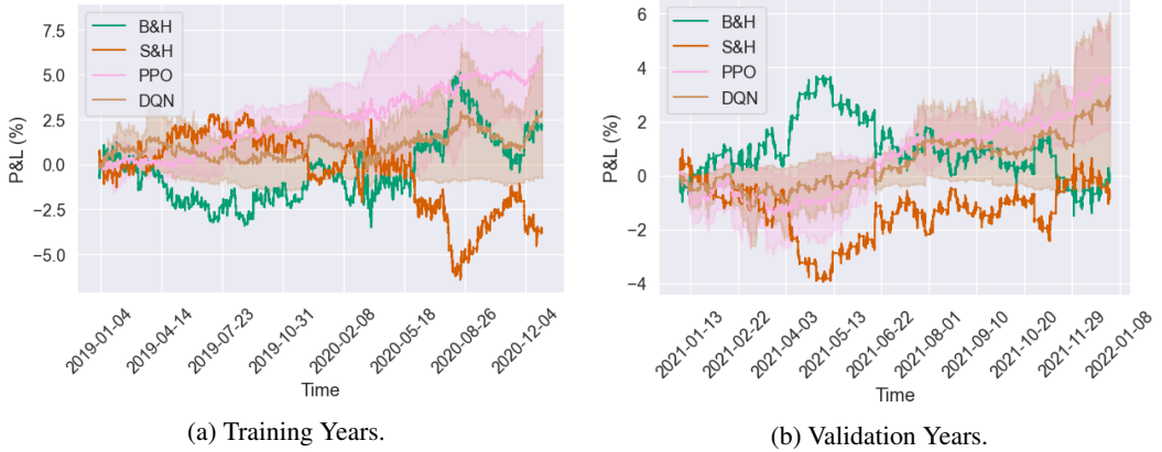
Figure 16: Performances of PPO and DQN w.r.t. common baselines (i.e., passive strategies) on Training (2019-2020) and Validation (2021) for TradingEnv. Confidence intervals obtained with 6 seeds.
