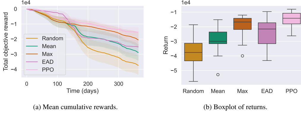
Figure 1: Performances of baselines in terms of mean cumulative reward (a) and average return (b) on DamEnv. Results are collected over 13 different episodes with a time horizon of one year.
