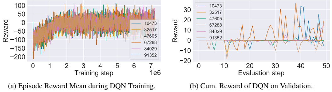
Figure 15: Training Curves DQN of the 6 seeds considered for TradingEnv, (a) episode reward mean on Training and (b) cumulative reward on the entire validation year.
