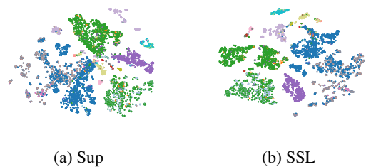
Figure 6: t-SNE visualization of representations with Pseudo labeling(SSL) and without(Sup). SSL achieves a better cluster results comparing with Sup, especially on color green and light purple.
