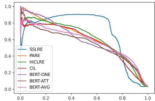
Figure 5: PR-curve
