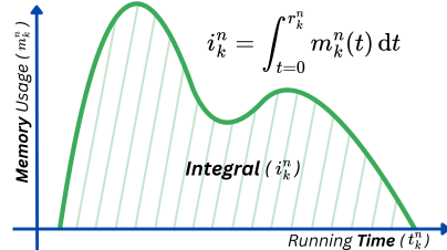
Figure 3: Illustration of task-level efficiency metrics.
