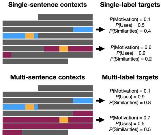
Figure 2: Shift in task form for citation context classification. Within a document (grey), each citation mention (orange) is associated with a surrounding context. Multi-sentence setting can contain both single-sentence (blue) and multi-sentence (purple) contexts. Multi-label scores need not sum to one as in the single-label setting.
