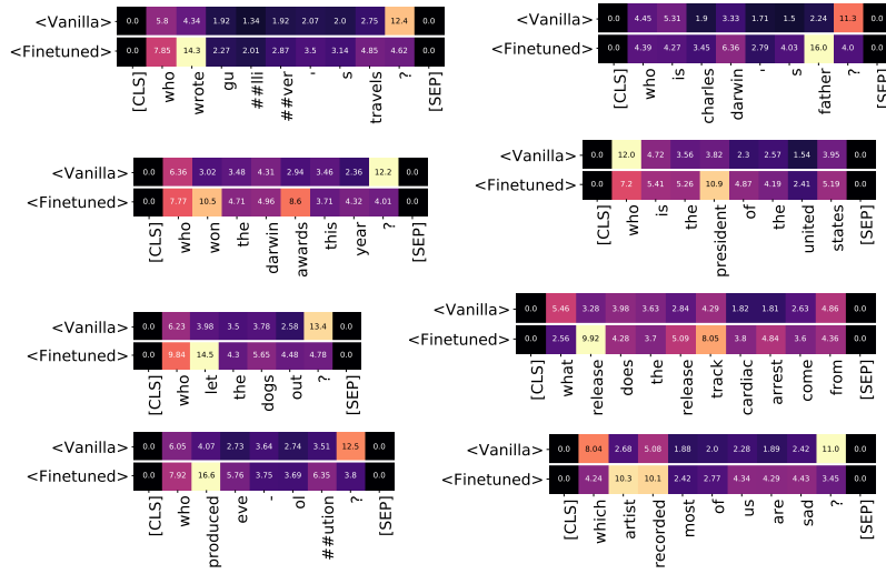
Fig. 2: Average of attention distributions for the [CLS] token for several examples. <Vanilla> is pretrained BERT before finetuning. <Finetuned> is BERT fine-tuned on our tasks.
