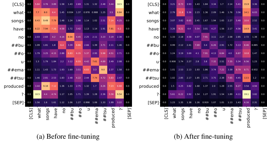
Fig. 1: Attention distributions averaged over all layers and attention heads for the example “What songs have Nobuo Uematsu produced?”, (a) before training on our tasks (vanilla pretrained BERT), and (b) after training on our tasks (finetuned BERT). We set the scores for [CLS] and [SEP] tokens to zero in the plots since they always receive a much higher average attention weight than the actual words from the sentence and thus would dominate the plot.
