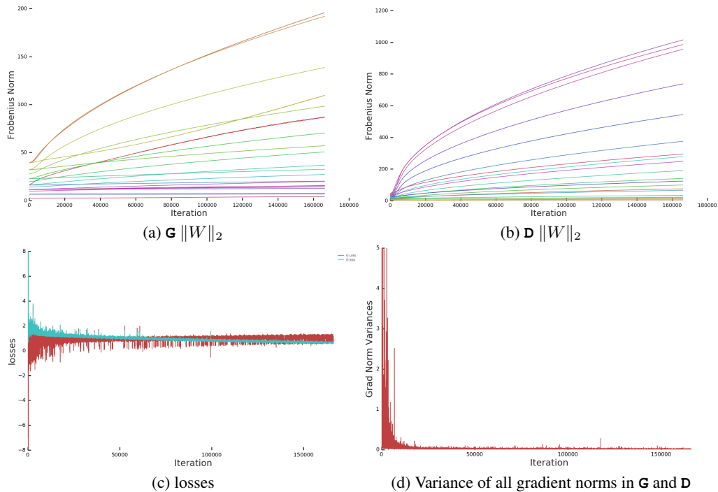
Figure 28: Additional training statistics with an R1 Gradient Penalty of strength 10 on \mathbf{D} . This model does not collapse, but only reaches a maximum IS of 55.
