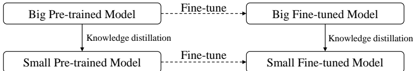
Figure 1: LightPAFF pipeline.
