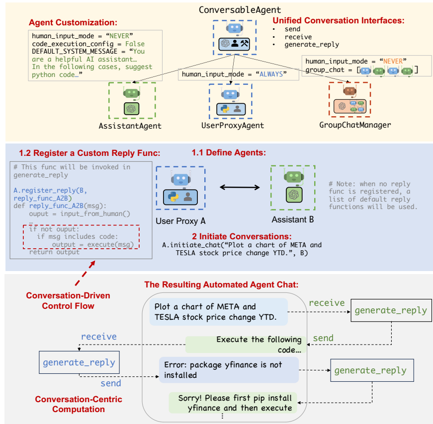
Figure 2: Illustration of how to use AutoGen to program a multi-agent conversation. The top sub-figure illustrates the built-in conversable agents provided by AutoGen. The middle sub-figure shows an example of using AutoGen to develop a two-agent system with a custom reply function. The bottom sub-figure illustrates the resulting automated agent chat from the two-agent system during program execution.
