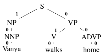
Figure 2: Yngve scoring
