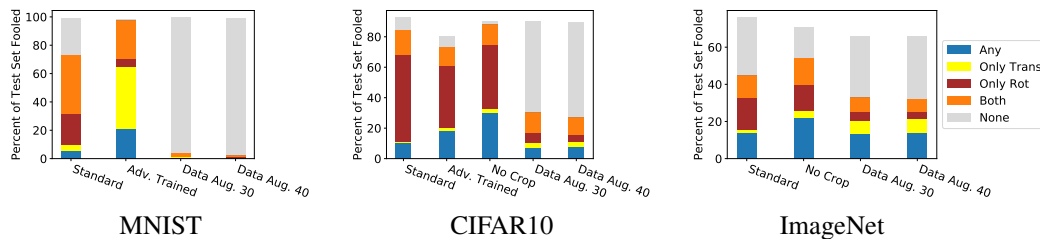
Figure 8: Fine-grained dataset analysis. For each model, we visualize what percent of the test set can be fooled via various methods. We compute how many examples can be fooled with either translations or rotations (“any”), how many can be fooled only by one of these, and how many require a combination to be fooled (“both”).
