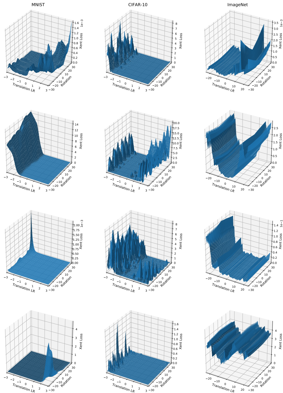
Figure 11: Loss landscape of 4 random examples for each dataset when performing left-right translations and rotations. Translations and rotations are restricted to 10% of the image pixels and 30^\circ respectively. We observe that the landscape is significantly non-concave, making rendering FO methods for adversarial example generation powerless.
