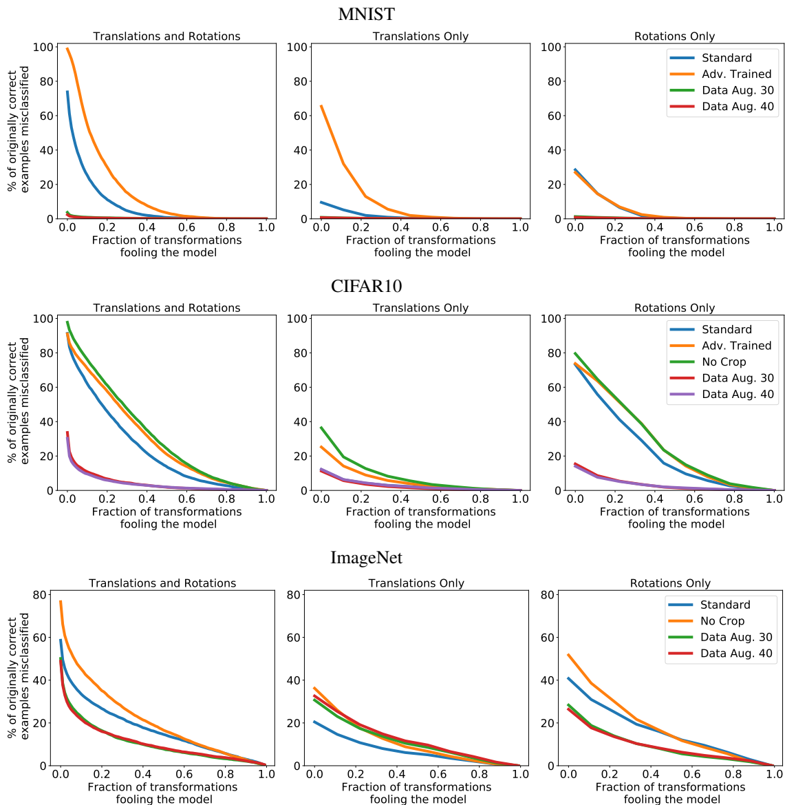
Figure 10: Cumulative Density Function plots. For each fraction of grid points p , we plot the percentage of correctly classified test set examples that are fooled by at least p of the grid points. For instance, we can see from the first plot, MNIST Translations and Rotations, that approximately 10% of the correctly classified natural examples are misclassified under 1/5 of the grid points transformations.
