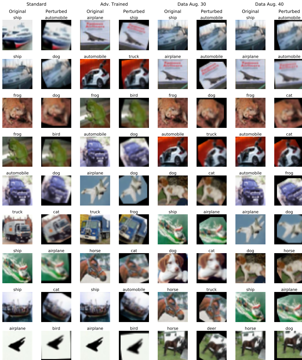
Figure 4: CIFAR10. Successful adversarial examples for the models studied in Section 4. Rotations are restricted to be within 30^\circ of the original and translations up to 3 pixels per directions (image size 32 \times 32 ). Each example is visualized along with its predicted label in the original and perturbed version.
