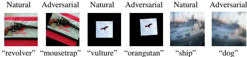
Figure 1: Examples of adversarial transformations and their predictions in the standard, "black canvas", and reflection padding setting.
