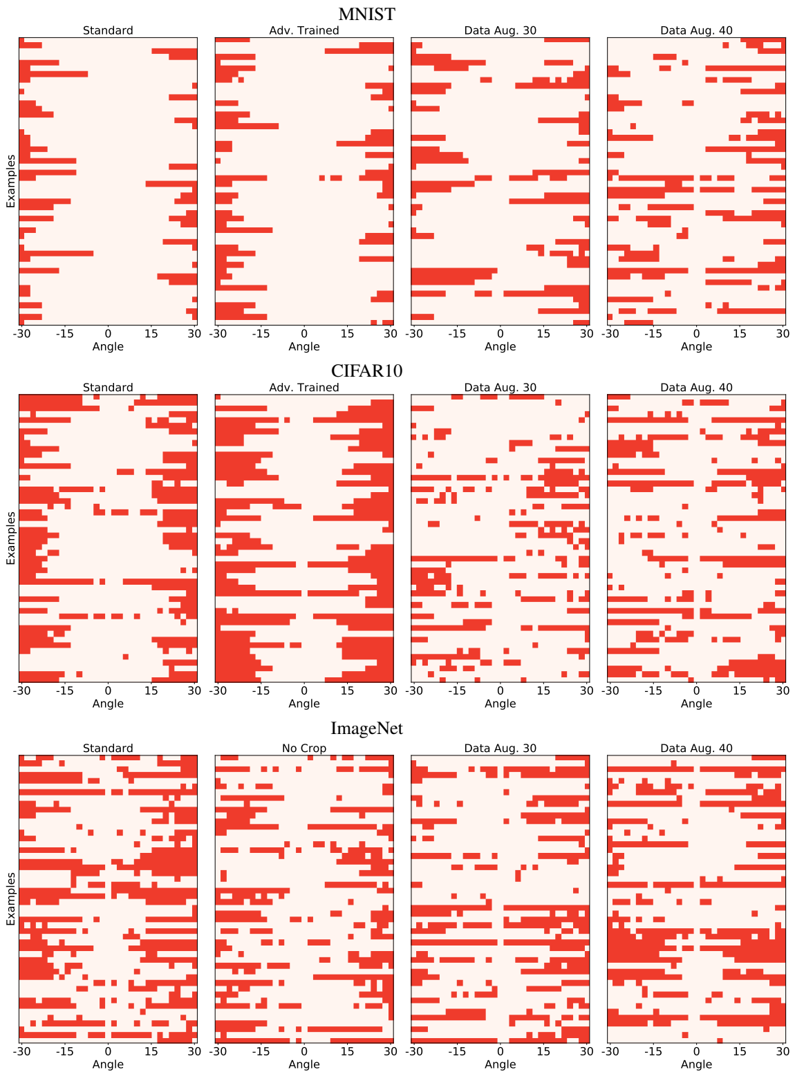
Figure 9: Visualizing which angles fool the classifier for 50 random examples. For each dataset and model, we visualize one example per row. Red corresponds to misclassification of the images. We observe that the angles fooling the models form a highly non-convex set.
