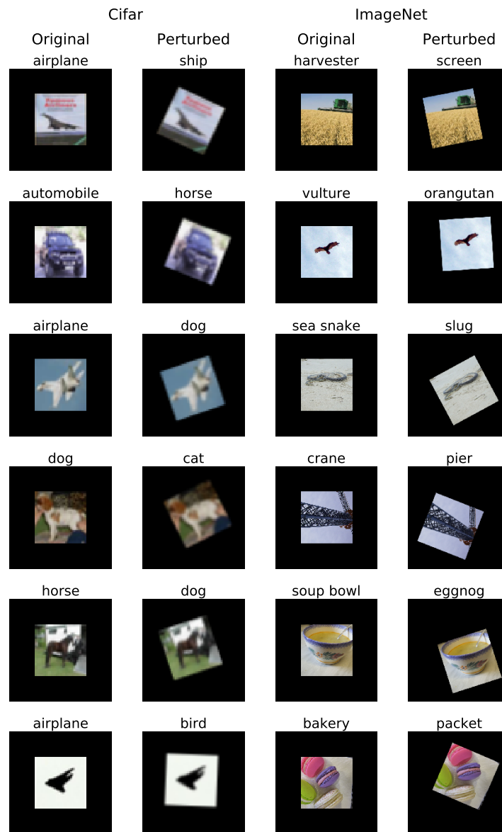
Figure 6: Sample adversarial transformations for the "black-canvas" setting for the standard models on CIFAR10 and ImageNet.
