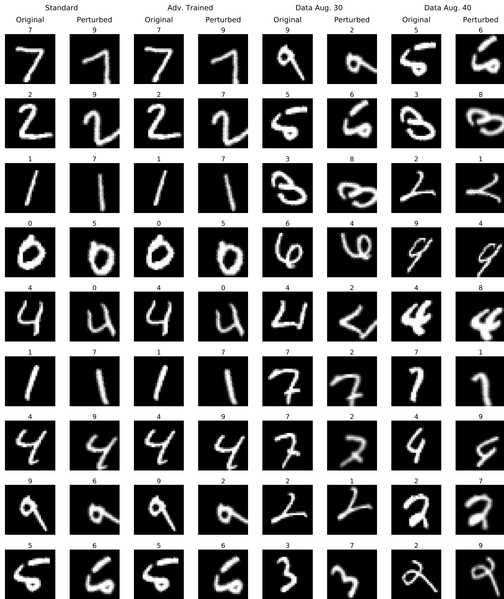
Figure 3: MNIST. Successful adversarial examples for the models studied in Section 4. Rotations are restricted to be within 30^\circ of the original image and translations up to 3 pixels per direction (image size 28 \times 28 ). Each example is visualized along with its predicted label in the original and perturbed versions.
