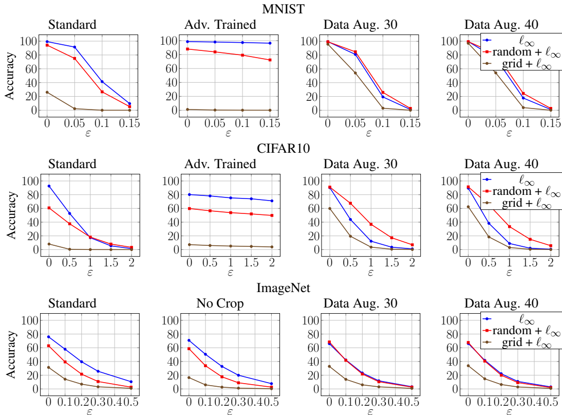
Figure 12: Accuracy of different classifiers against \ell_\infty -bounded adversaries with various values of \epsilon and spatial transformations. For each value of \epsilon , we perform PGD to find the most adversarial \ell_\infty -bounded perturbation. Additionally, we combine PGD with random rotations and translations and with a grid search over rotations and translations in order to find the transformation that combines with PGD in the most adversarial way.
