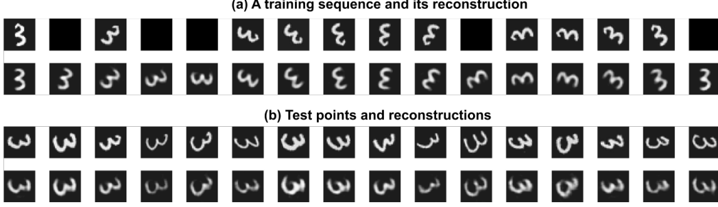
Figure 4: Panel (a) shows a training sequence with missing values (first row) and its reconstruction (second row). First row in panel (b) demonstrates test angles from different sequences, i.e., hand-writing styles, and below are model predictions.
