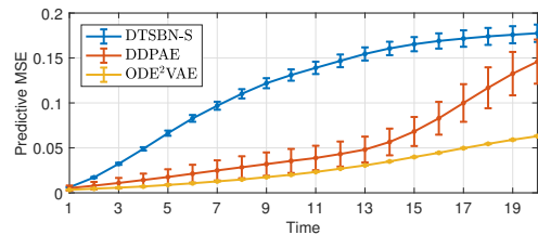
Figure 3: Bouncing balls errors.
