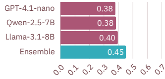
(a) Weak judges ensemble (tau-c)
