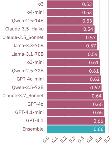
(b) Strong judges ensemble (tau-c)
