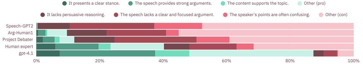
Figure 16: Distribution of the top three pro and con key points in Qwen-32B ’s chain-of-thought explanations, grouped by source. Other (pro) and Other (con) denote less frequent points. The relative share of positive key points per source reflects the judge ratings discussed in Sections 5.2 and 5.3
