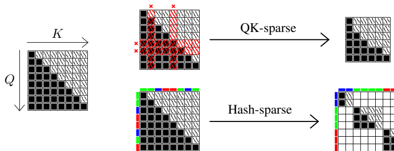
Figure 1. Sparsification of the attention matrix. In each depicted attention matrix, black areas indicate coefficients to compute, patterned areas those forced to zero due to the causal masking, and white areas coefficients that are ignored. We consider two dynamic strategies to sparsify the left attention matrix. The QK-sparse attention consists of dropping some keys and queries (top, the discarded keys and queries are indicated in red), and the Hash-sparse attention computes a hash code for each key and each query, and restricts the attention matrix to blocks of keys and queries of same hash code (bottom, the three hash values are indicated for each key or query with the colors blue/green/red). In both cases, the attention operation must be able to deal with sub-blocks of the attention matrix with a non-triangular causal mask.
