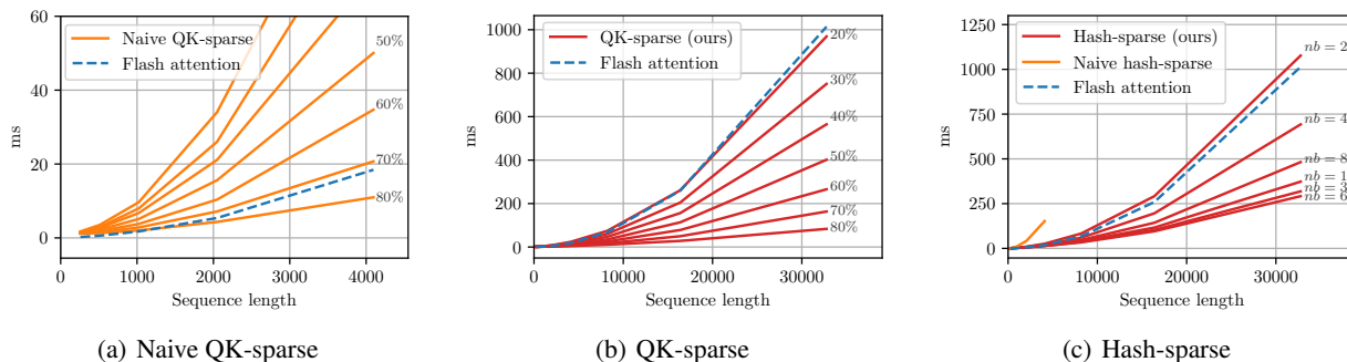
Figure 2. Fig.(a) & Fig.(b): Runtimes of full Flash-attention (Dao et al., 2022) and Query/Key dropping based sparsity. We show the forward + backward runtimes. For sparse methods, we drop at random a percentage of keys and queries. Fig.(a): A naive implementation consisting in creating compact representations of the key, value, and query tensors by removing dropped keys and queries. As a result, the attention matrix is no longer triangular (see Fig. 1). We call the PyTorch scaled_dot_product_attention method with a custom but still causal mask. The non-triangular mask prevents FlashAttention to be used and only dropping more than 70% of the keys and queries seems to improve the runtime over attending the entire sequence using FlashAttention. Fig.(b): Our modification of FlashAttention improves the runtime. Reshaping the tensor induces an overhead which compensates the speed gain for shorter sequences. However, this offset is compensated by a strong margin as the sequence length increases. Our implementation allows significant gains over FlashAttention even for low levels of sparsity. The detailed runtimes for the forward and backward passes can be found in App. C. Fig.(c): Runtimes of the full Flash-attention and hash-based sparsity. Similarly to our QK-sparse method we show how a naive implementation fails to provide any speed gain. On the other hand, our modification of the basic FlashAttention method computes only what is required. While there is a cost to reordering the tensors based on the hash buckets, this cost is largely compensated for as the number of buckets nb increases, and as the sequence length increases.
