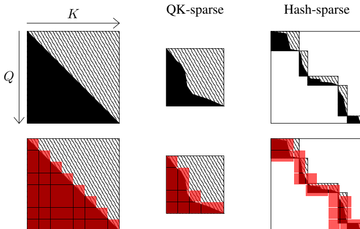
Figure 4. SCFA computation patterns. In each depicted attention matrix, black areas indicate coefficients to compute, patterned areas are those forced to zero due to the causal masking, and white areas coefficients that are ignored. The red squares in the bottom matrices show the tiles actually computed by our SCFA kernel. In the regular case (left), this coincides with the behavior of FlashAttention. However, in the case of irregular causal masking due to keys/queries dropping (center) or in the case of irregular causal masking and band block sparsity due to hashing (right), FlashAttention does not provide means to compute a fine-grain subset of the attention matrix.
