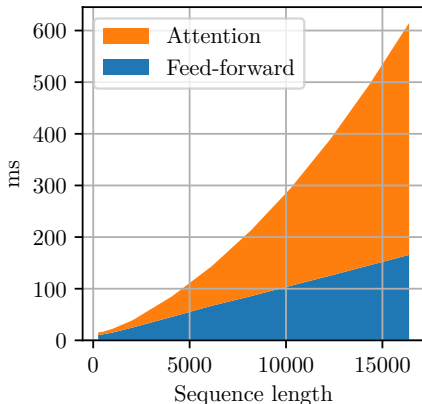
Figure 5. Quadratic computational cost of self attention dominates for larger sequences. We measure the forward and backward runtimes for a 12 layers transformer (see App. B.4 for implementation details). Except for the attention operations, the rest of the transformer runtime grows linearly with the sequence length.
