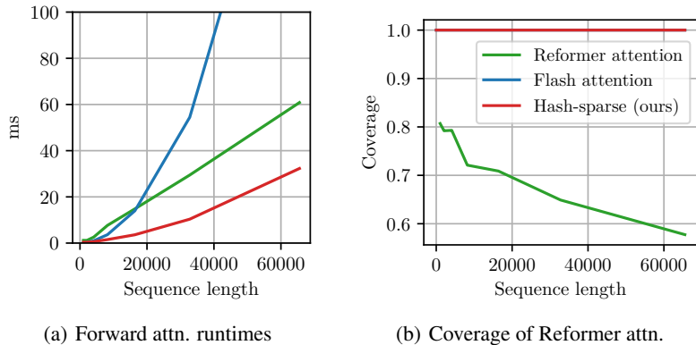
Figure 13. Comparing forward runtimes of attention modules alone. Fig.(a): Reformer attention ensures a linear computational complexity w.r.t. the sequence length, outperforming FlashAttention for longer sequences. Fig.(b): However, due to the fixed attention structure, the Reformer misses an increasing fraction of hash collisions. Our approach outperforms both methods and maintains 100% exact coverage of collisions for all sequence lengths. See App. B.4 and App. C for more details.
