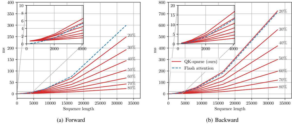
Figure 7. Forward and Backward runtimes in a vacuum for our QK-sparse method. Fig.(a) Forward runtimes for our QK-sparse method. Fig.(b): Backward runtimes for our QK-sparse method.
