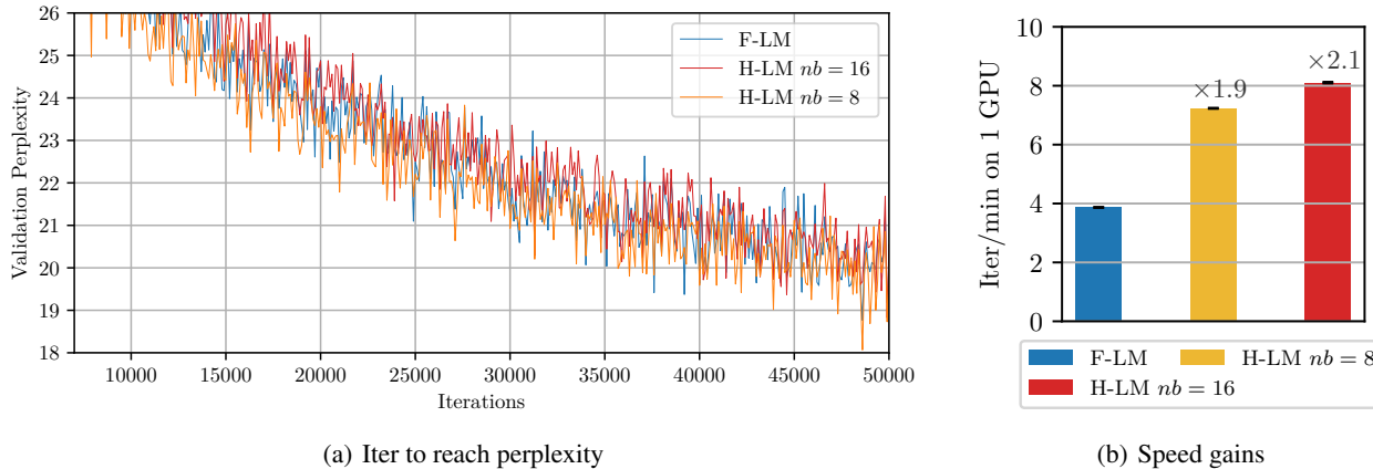
Figure 12. Comparison between H-LM and F-LM when training for 50k iterations on sequences of 8192 tokens. Those curves are averaged over two seeds. In Fig.(a) we zoom in on the perplexity per iteration for the baseline F-LM and two of our H-LM models using our Hash-sparse attention with 8 and 16 buckets. We observe that our methods are matching the perplexity of the F-LM model which uses FlashAttention over the entire sequence. Fig.(b): We match the perplexity but gain in speed, our methods are 1.4\times and 1.8\times faster than the baseline for respectively 8 and 16 buckets.
