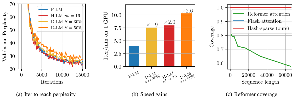
Figure 3. Fig.(a) & Fig.(b): Training Language Models (LM) on OpenWebText2 (Gao et al., 2020) using Hash-sparse (H-LM), QK-sparse (D-LM), or FlashAttention over the entire sequence (F-LM). We train on sequences of length 8192 and use 16 buckets for our H-LM model and a sparsity of 30% and 50% for our D-LM models. We show that it is possible to use our proposed dynamic sparsity schemes to significantly gain in speed (Fig.(b)) without compromising the perplexity (Fig.(a)). In Fig.(c) we observe the impact of the fixed attention structure in Reformer: an increasing fraction of hash collisions are missed. Our approach maintains 100% exact coverage of collisions for all sequence lengths. See App. C for more details.
