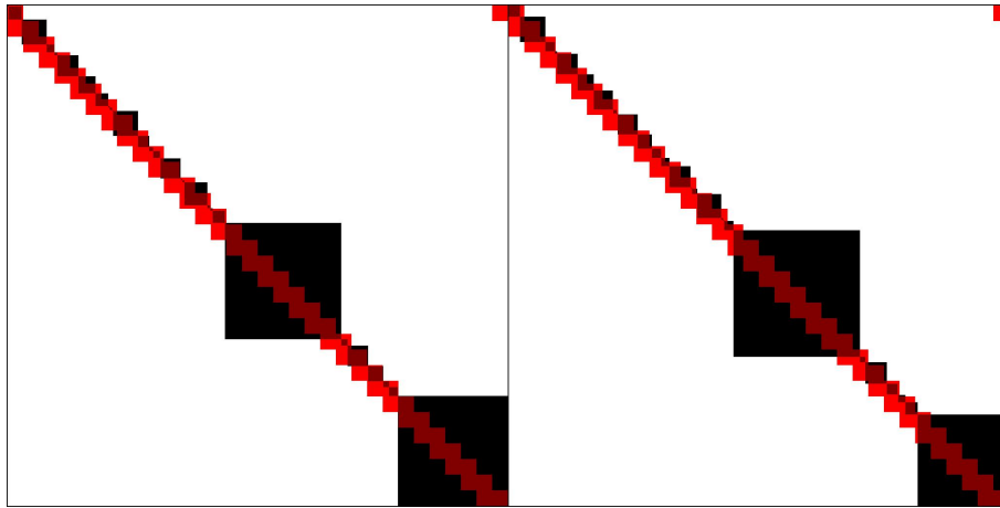
Figure 15. Attention pattern of Reformer. The two images show the attention pattern for the Reformer LSH attention after reordering queries and keys according to the bucket. The red squares are the positions for which attention is computed in the Reformer with bucket size = 32. The black squares are positions for which the queries and keys map to the same hash bucket. Queries are sampled from a normal distribution with \mu = 3 and \sqrt{\sigma} = 5 . Each image refers to a different attention head. Black regions which are not covered by red tiles are key-query interactions which should be computed but are missed by the Reformer LSH attention.
