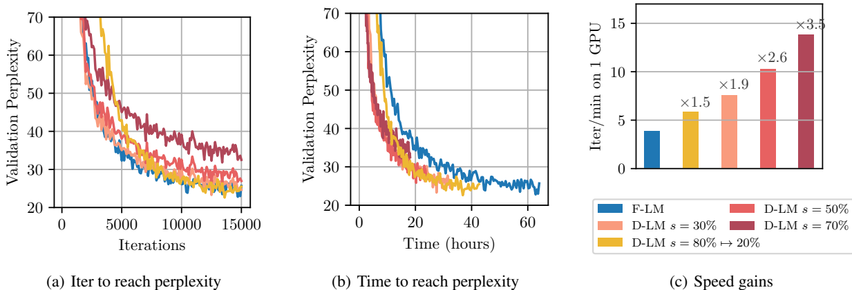
Figure 9. Training Language Models (LM) on OpenWebText2 using random Query/Key dropping based sparsity (D-LM) or FlashAttention over the entire sequence (F-LM). We include the D-LM model with linear decay of s from 80% to 20%. In Fig.(b) and Fig.(c), we observe the additional D-LM model in yellow is slower than other D-LM models we experimented with, but, as seen in Fig.(a), reaches a slightly better perplexity.
