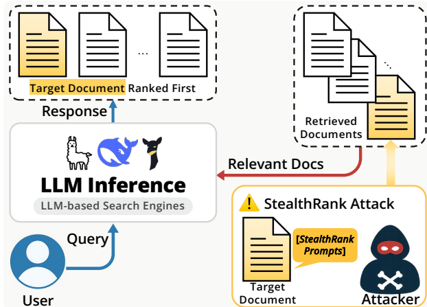
Figure 1. Overview of the LLM-based ranking attack pipeline. Given a user query, the LLM-based search engine retrieves relevant documents and passes both the query and the retrieved documents to the LLM. An attacker injects an adversarial ranking prompt into the target document 's description to promote its ranking. The manipulated list is then processed by the LLM, resulting in a response where the target document is ranked higher while the ranking prompt remains stealthy.
