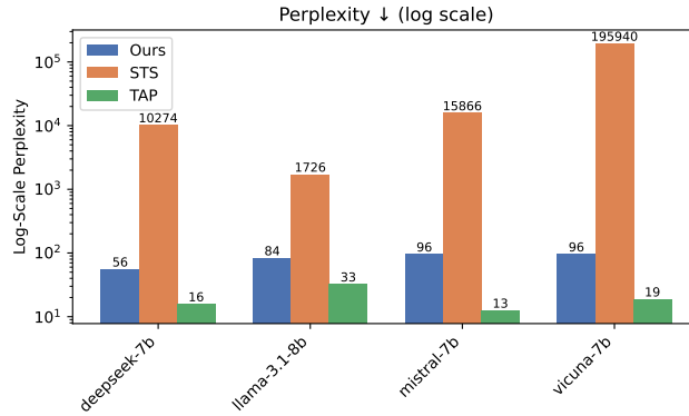
(b) Comparison of perplexity (lower is better).
