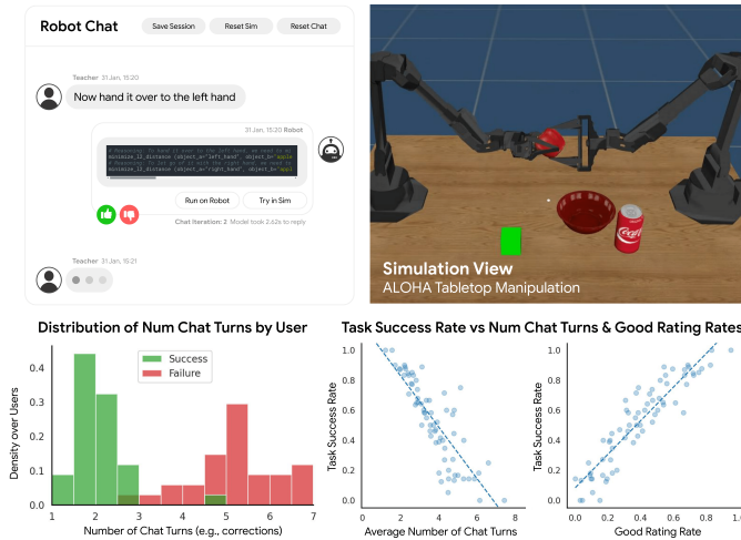
Fig. 3: Our chat interface (top left) allows non-experts to use language to teach robots new behaviors (visualized in simulation, top right). Our LLM responds with reward code, to drive real-time motion control of a simulated or real robot. Statistics show that base model data meets expectations: successful teaching sessions take fewer chat turns than failures (bottom left), and task success rates correlate with fewer chat turns ( r = -0.85 , bottom middle) and higher good rating rates (i.e., responsiveness to feedback, r = 0.92 , bottom right).
