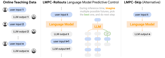
Fig. 4: Given a dataset of users teaching robots new tasks with language (represented as text inputs and code outputs from online in-context learning – left), LMPC-Rollouts is trained to predict subsequent inputs and outputs conditioned on the current chat history (middle), and uses MPC (receding horizon control) for inference-time search to return the next best action (with fewest expected corrections before success). LMPC-Skip is an alternate variant that is trained to directly predict the last action (right). Both LMPC variants accelerate fast robot adaptation via in-context learning.
