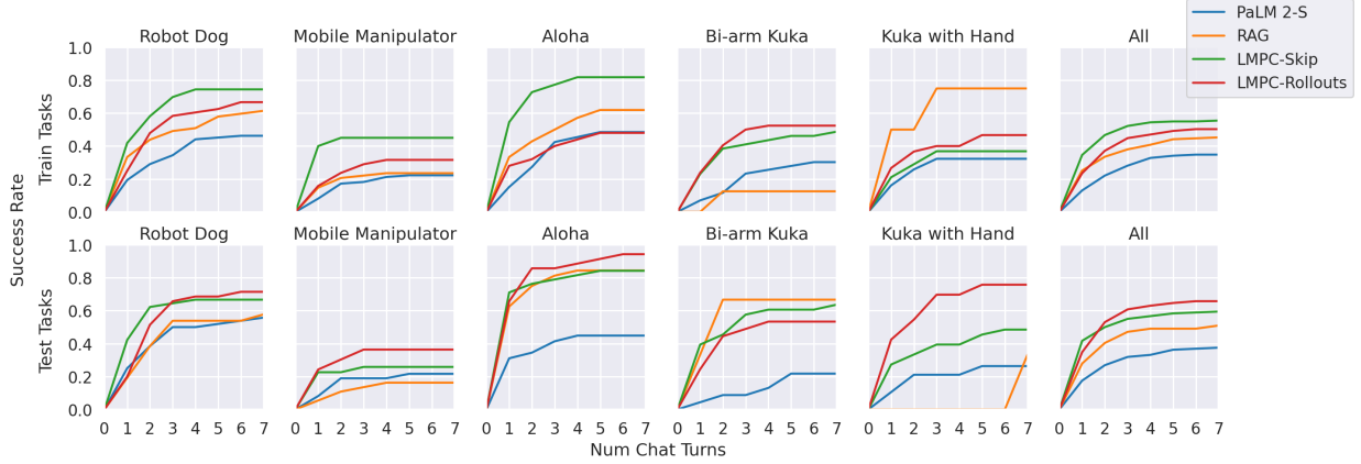
Fig. 8: Task Success vs. Number of Chat Turns. across embodiments
