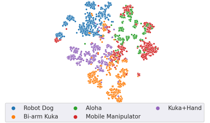
Fig. 12: T-SNE plot of embeddings of human feedback across embodiment.
