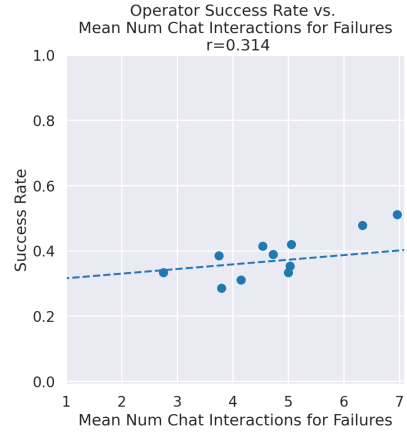
Fig. 6: Correlation of Operator Success Rate and Num Chat Turns until Failures
