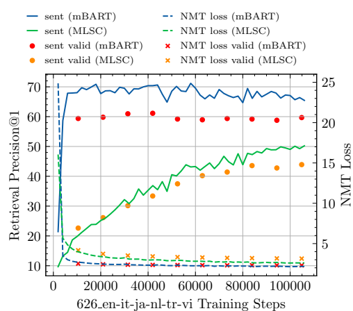
Figure 1: NMT loss, sentence retrieval P@1 of the encoder in MLSC and mBART FT. The average of the contextual embeddings on top of the encoder is used as the sentence embedding. We report the average in-batch retrieval precision of both directions of each language pair.
