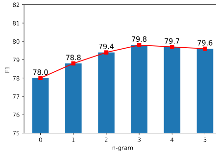
Figure 3: Performance on Tacred Revisited test set with different n-gram segments features. Number n in x-axis means the model use n -gram segment features.
