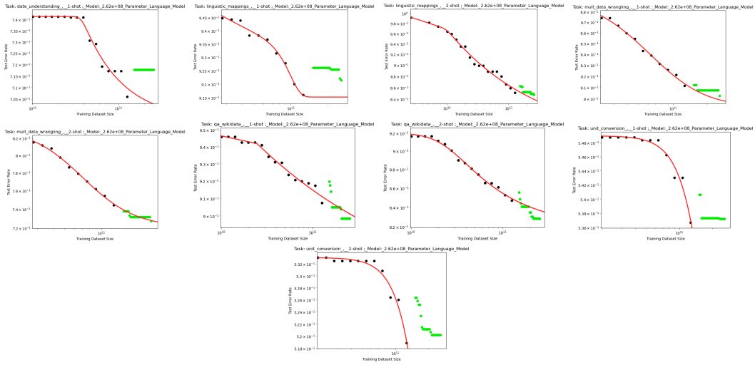
Figure 13: BIG-Bench (BB). From eyeballing, we think the subset of BIG-Bench with unsatisfactory extrapolations has unsatisfactory extrapolations due to the maximum (along the x-axis) of the black point used for fitting being near or before a break; this is accentuated by not having enough points for fitting for the SciPy fitter to be able to determine whether the break is an actual break or just noisy deviation.
