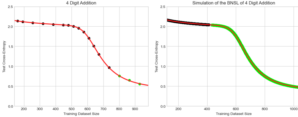
Figure 2: 4 Digit Addition. Note that these plots are linear-linear. Each point in the left plot is the mean of greater than 1000 seeds at that dataset size. In the left plot, each point is gathered from a model trained to do the task of 4-digit addition. In the right plot, each point is gathered from a noiseless simulation of the BNSL of the task of 4-digit addition.
