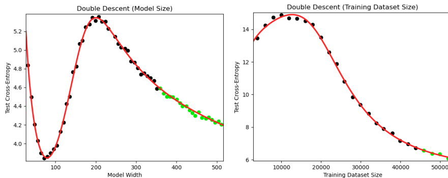
Figure 5: Extrapolation of BNSL on Double Descent. Both plots are of transformers trained to do neural machine translation via minimizing cross-entropy. Experimental data of left figure is obtained from Figure 8 top of Nakkiran et al. (2021); “Model Width” on the x-axis refers to embedding dimension d_{model} of the transformer. Experimental data of the right figure is obtained from Figure 11b of Nakkiran et al. (2021). The plot on the left contains two breaks of a BNSL fit to the black points. See Section C.5 for more details.
