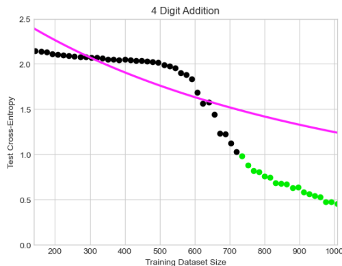
Figure 3: 4 Digit Addition. Fit of M3 (functional form that can't express inflection point) to 4 digit addition.
