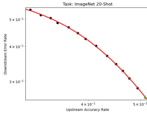
Figure 7: Extrapolation Results of BNSL for scaling behavior when Upstream Performance is on the x-axis and Downstream Performance is on the y-axis. Experimental data of scaling behavior obtained from Figure 5 of Abnar et al. (2021). The upstream task is supervised pretraining of ViT (Dosovitskiy et al., 2020) on subsets of JFT-300M (Sun et al., 2017). The Downstream Task is 20-shot ImageNet classification. See Section C.10 for more details.
