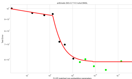
Figure 4: Large-Scale BIG-Bench Arithmetic. Extrapolation yielded by BNSL on BIG-Bench 3-shot Arithmetic task with number of parameters on the x-axis. This experimental data is obtained from the Srivastava et al. (2022) release.
