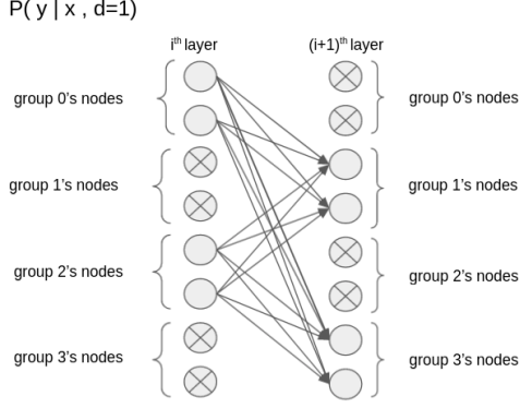
Figure 1: Latent group dropout. The set of nodes in each layer is divided into equal-sized groups. For each task, we only keep a fixed number of active groups of nodes and nullify all the other nodes.
