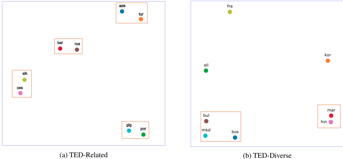
Figure 3: Visualization of languages according to their dropout masks (a large vector concatenating the dropping masks of all the layers of the model) constructed by PCA.
