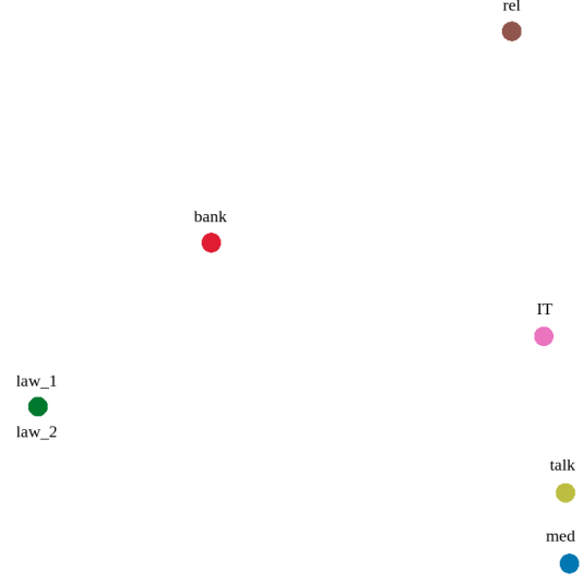
Figure 4: Visualization of domains according to their dropout masks (a large vector concatenating the dropping masks of all the layers of the model) constructed by PCA.
