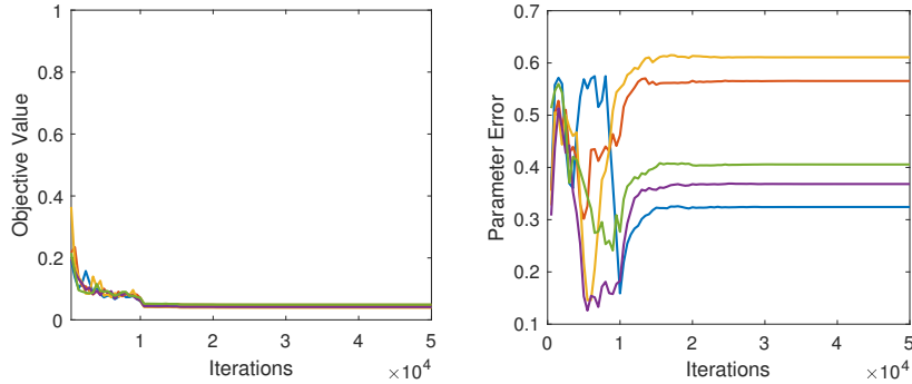
Figure 2: Data are generated by a network with sigmoid activation without noise. The training model uses the same architecture. Left: the estimated population risk doesn’t converge to zero. Right: the parameter error using the surrogate in equation (4.1).
