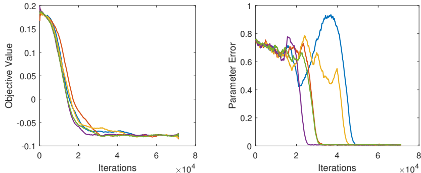
Figure 4: Learning with objective function G(\cdot) . Left: the test loss. Right: the error in parameter space measured by equation (4.1)
