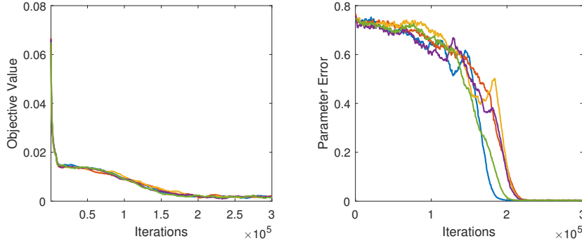
Figure 3: The labels are generated from a network with ReLU activation. We learn with \hat{\sigma}_2 h_2 + \hat{\sigma}_4 h_4 activation. Left: the test loss subtracted by the theoretical global minimum value. Right: the error in parameter space measured by equation (4.1)
