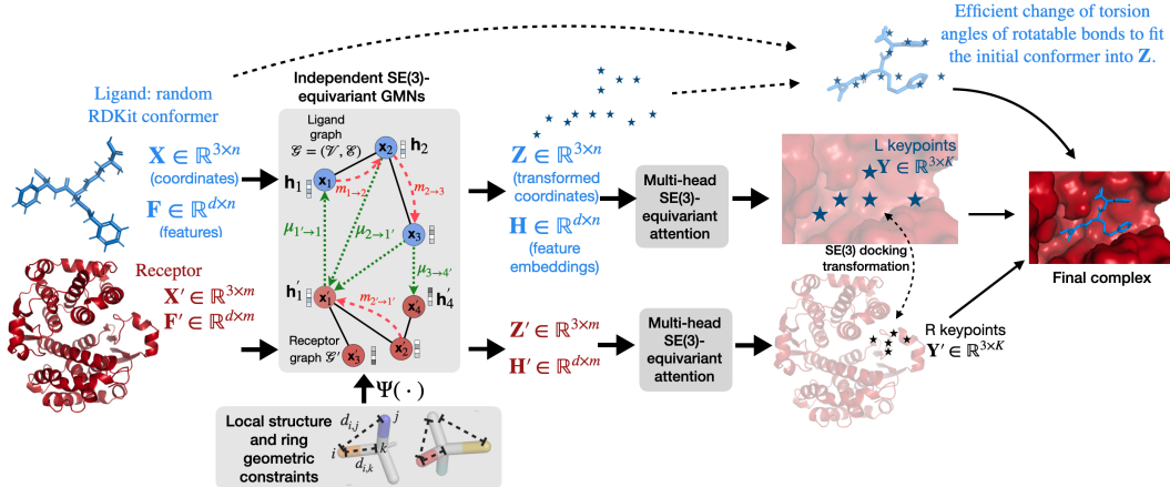
Figure 15: EQUIBIND model architecture.
