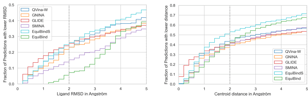
Figure 9: Flexible blind self-docking. Zoomed in versions of the histograms in Figure 2 where only the 0-5 Å range is shown. Left: Cumulative histogram of the L-RMSD. Right: Cumulative histogram of the centroid distance.
