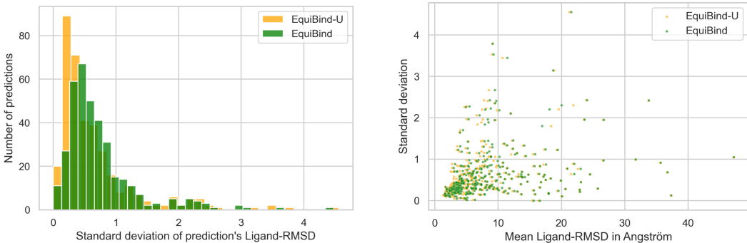
Figure 7: Sensitivity to initial conformer. Left: Histogram of the standard deviations of the L-RMSDs of EQUIBIND's and EQUIBIND-U's predictions when using 30 different initial conformers. Right: Scatter-plot with a point for each complex showing the mean L-RMSD and standard deviation of EQUIBIND's or EQUIBIND-U's 30 predictions from 30 different initial input conformers.
