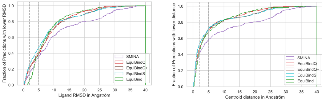
Figure 6: Flexible blind self-docking. Left: Cumulative histogram of the L-RMSD. Right: Cumulative histogram of the centroid distance.
