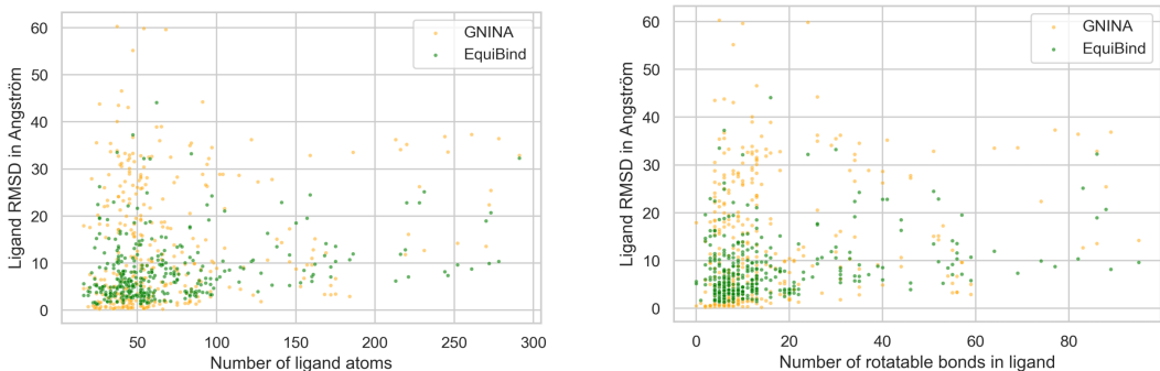
Figure 8: Performance correlation with molecule size. Left: Scatter-plot showing the L-RMSD and the number of ligand atoms for each prediction of EQUIBIND and GNINA. Right: The same for the number of rotatable bonds in the ligand.
