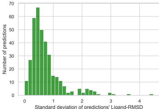
Figure 4: Histogram of the standard deviations of the L-RMSDs of EQUIBIND’s predictions when using different initial conformers.
