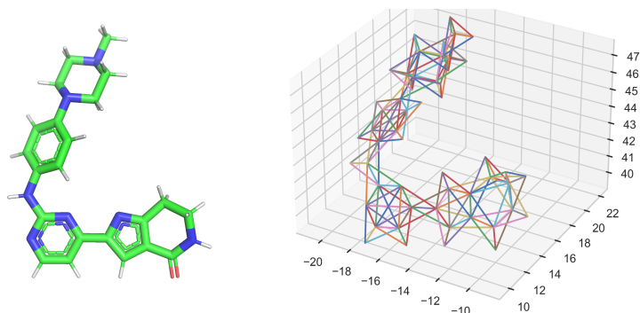
Figure 11: LAS distance geometry constraint visualization. Visualization of the interatomic distances which are included in the LAS distance geometry constraints in Equation 2.2. The pairwise distances in rings are only included if the ring is aromatic, like in the bottom left ring of the depicted molecule. The torsion angles in non-aromatic rings, such as the one in the bottom right, remain flexible.
