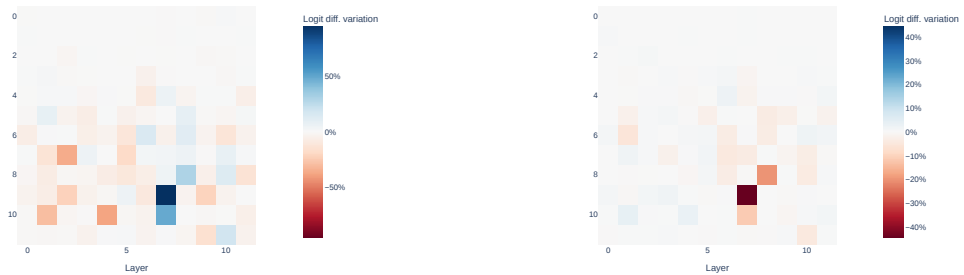
(a) Simple Syllogism with Positive/Negative
