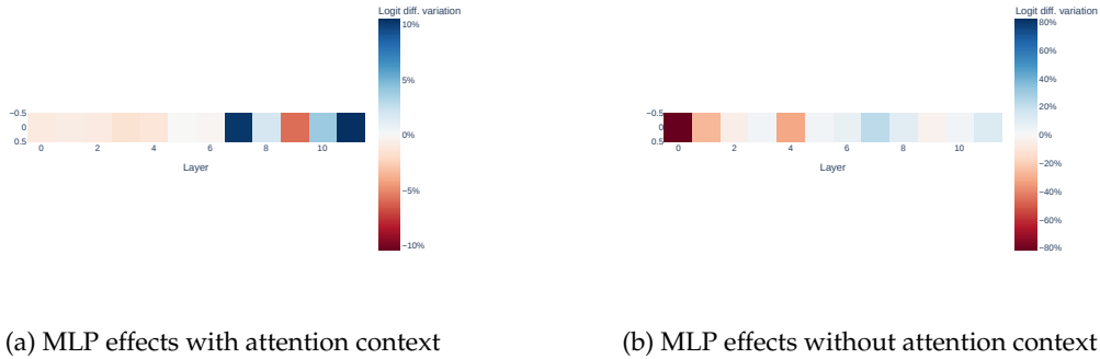
Figure 10: Path patching MLPs in the simple syllogism task. (a) shows effects when MLPs are patched with attention context preserved. No MLPs have significant importance; (b) shows isolated MLP contributions without attention context. Early MLPs, specifically MLP0, appear relevant for the task
