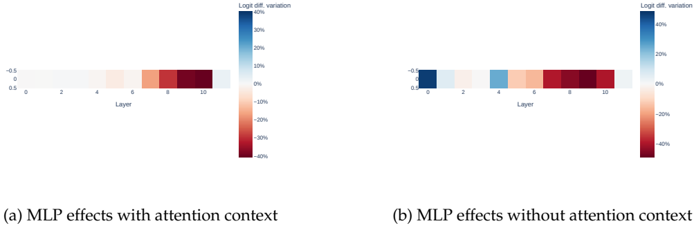
Figure 9: Path patching MLPs in the opposite syllogism task. (a) shows effects when MLPs are patched with attention context preserved; (b) shows isolated MLP contributions without attention context.
