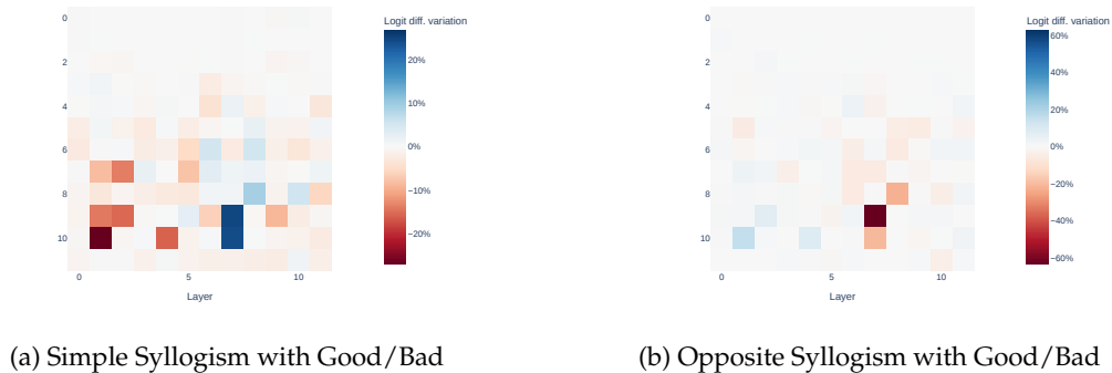
Figure 8: Binary task results of Good/Bad
