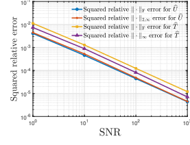
Figure 3: Squared relative errors vs. SNR for noisy settings. Here, d = 100 , r = 4 , p = 0.1 . Each point is averaged over 100 trials.
