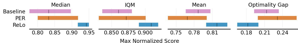
Figure 2: Metrics aggregated across 9 environments and 5 seeds in DMC based on proposed metrics from Agarwal et al. [2021]
