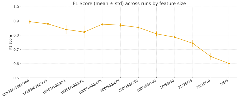
Figure 6: F1-score (mean \pm std) across five runs by feature size. Error bars denote standard deviation.
