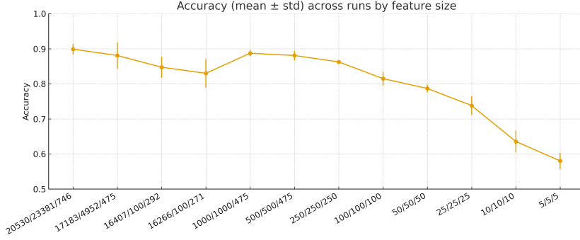
Figure 5: Accuracy (mean \pm std) across five runs by feature size. Error bars denote standard deviation. Following this preprocessing, our final dataset consisted of:
